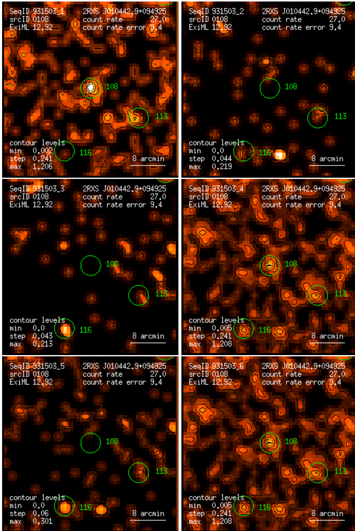
Figure 108: RASS 931503: detection 0108: band rate images, Gaussian filter: (1) PSPC channels 11 – 41, (2) 52 – 90, (3) 91 – 201, (4) 11 – 235, (5) 52 – 201, (6) 11 – 201. Broad band rates in counts/ks. Band rate contour levels in counts/ks/arcmin 2 .
