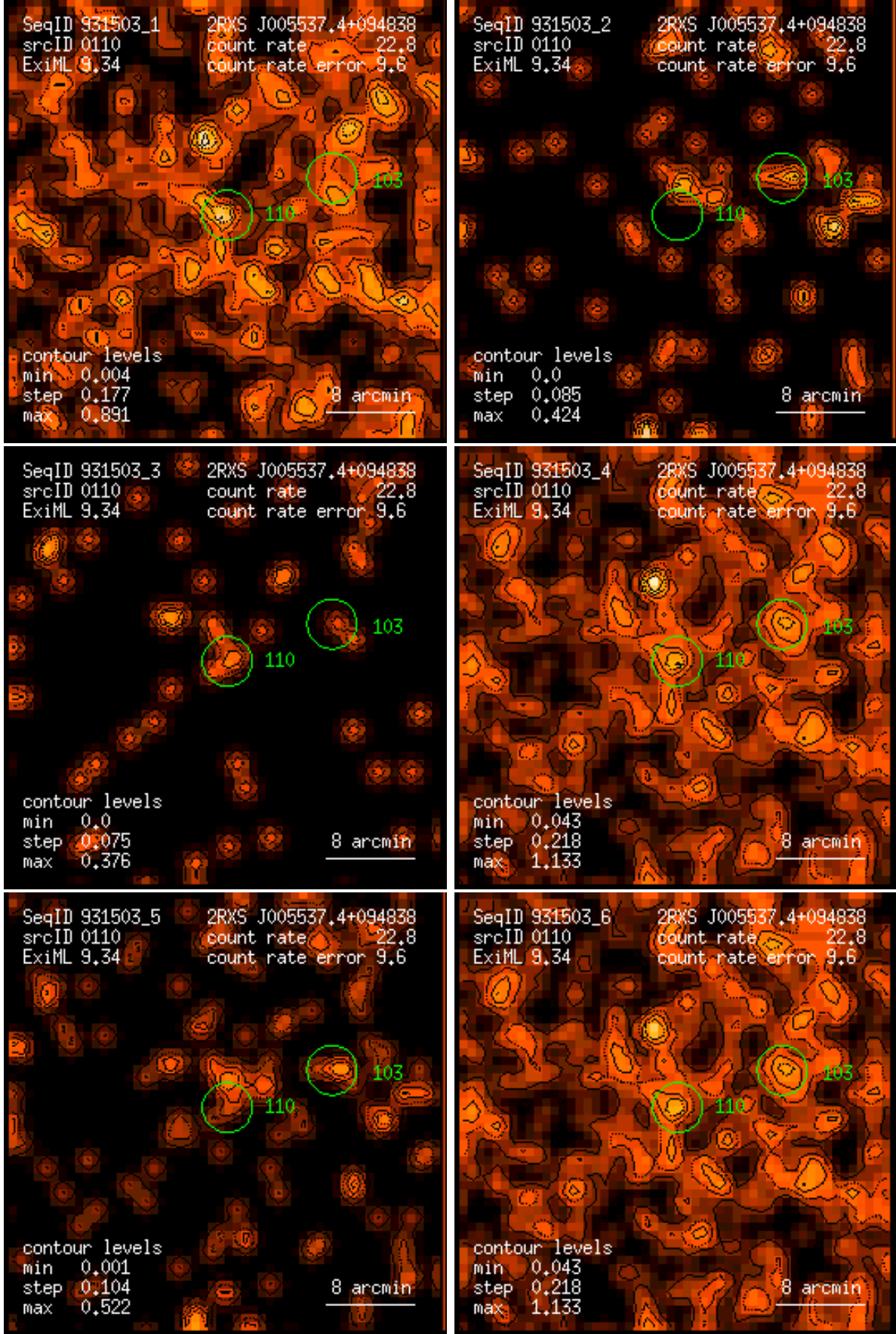
Figure 110: RASS 931503: detection 0110: band rate images, Gaussian filter: (1) PSPC channels 11 – 41, (2) 52 – 90, (3) 91 – 201, (4) 11 – 235, (5) 52 – 201, (6) 11 – 201. Broad band rates in counts/ks. Band rate contour levels in counts/ks/arcmin 2 .
