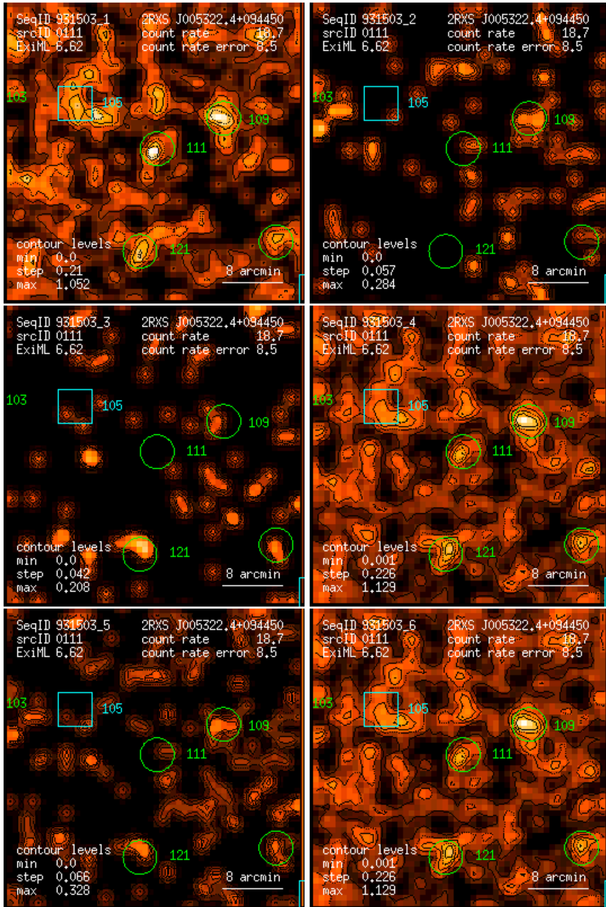
Figure 111: RASS 931503: detection 0111: band rate images, Gaussian filter: (1) PSPC channels 11 – 41, (2) 52 – 90, (3) 91 – 201, (4) 11 – 235, (5) 52 – 201, (6) 11 – 201. Broad band rates in counts/ks. Band rate contour levels in counts/ks/arcmin 2 .
