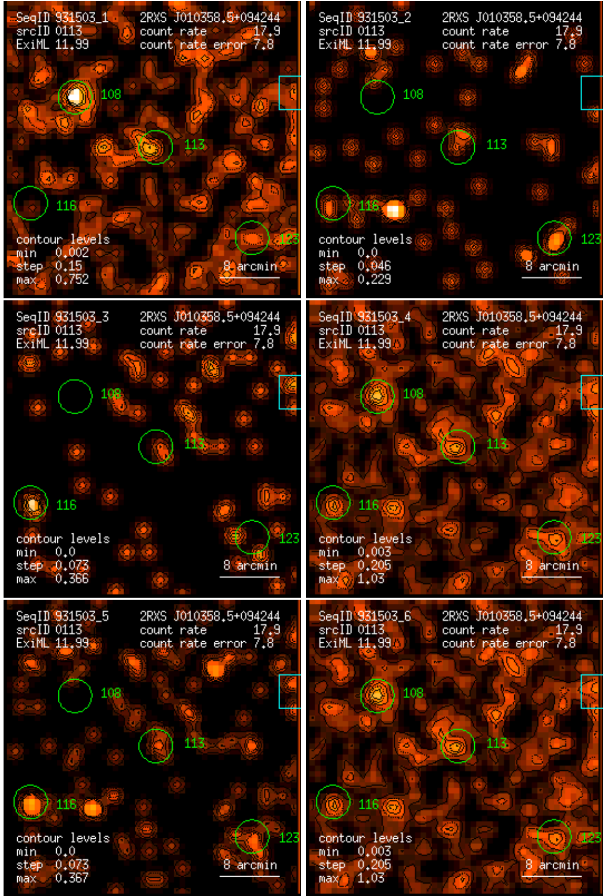
Figure 113: RASS 931503: detection 0113: band rate images, Gaussian filter: (1) PSPC channels 11 – 41, (2) 52 – 90, (3) 91 – 201, (4) 11 – 235, (5) 52 – 201, (6) 11 – 201. Broad band rates in counts/ks. Band rate contour levels in counts/ks/arcmin 2 .
