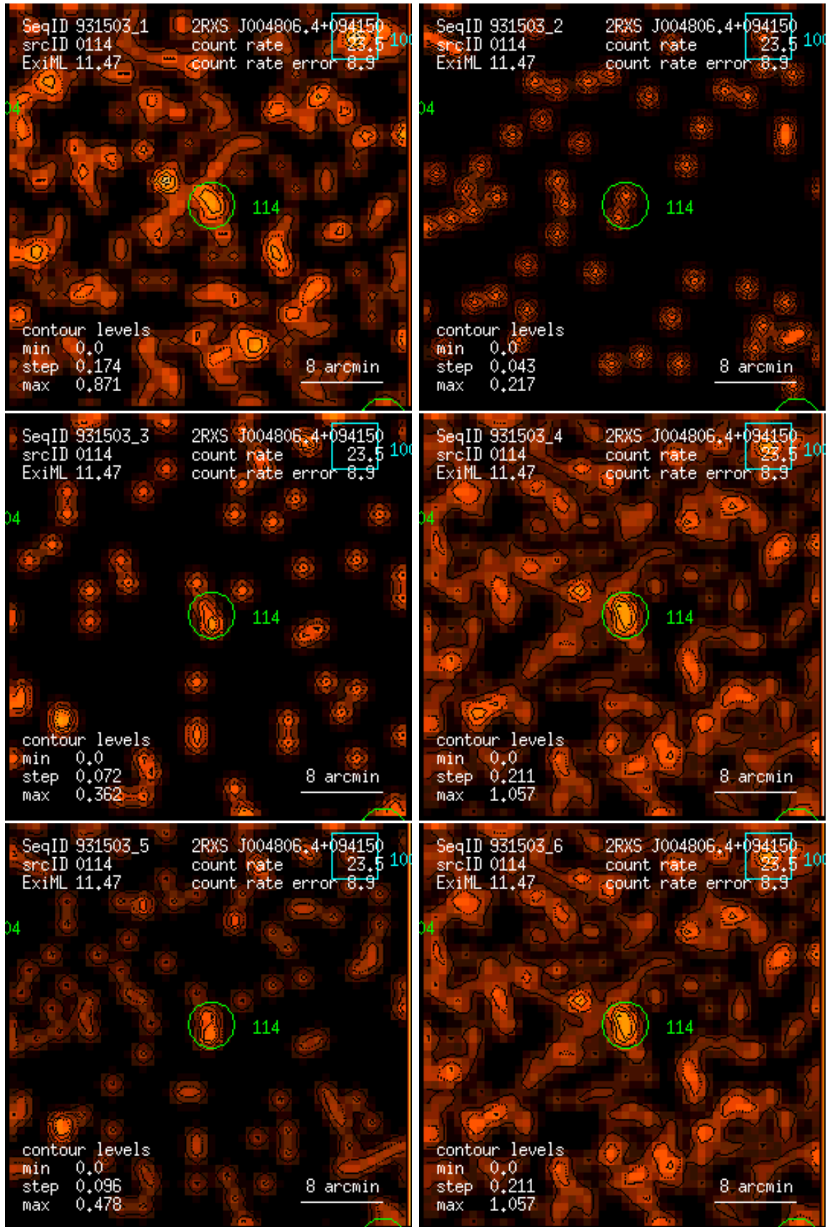
Figure 114: RASS 931503: detection 0114: band rate images, Gaussian filter: (1) PSPC channels 11 – 41, (2) 52 – 90, (3) 91 – 201, (4) 11 – 235, (5) 52 – 201, (6) 11 – 201. Broad band rates in counts/ks. Band rate contour levels in counts/ks/arcmin 2 .
