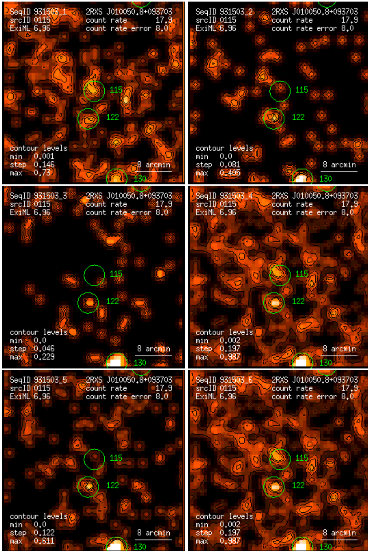
Figure 115: RASS 931503: detection 0115: band rate images, Gaussian filter: (1) PSPC channels 11 – 41, (2) 52 – 90, (3) 91 – 201, (4) 11 – 235, (5) 52 – 201, (6) 11 – 201. Broad band rates in counts/ks. Band rate contour levels in counts/ks/arcmin 2 .
