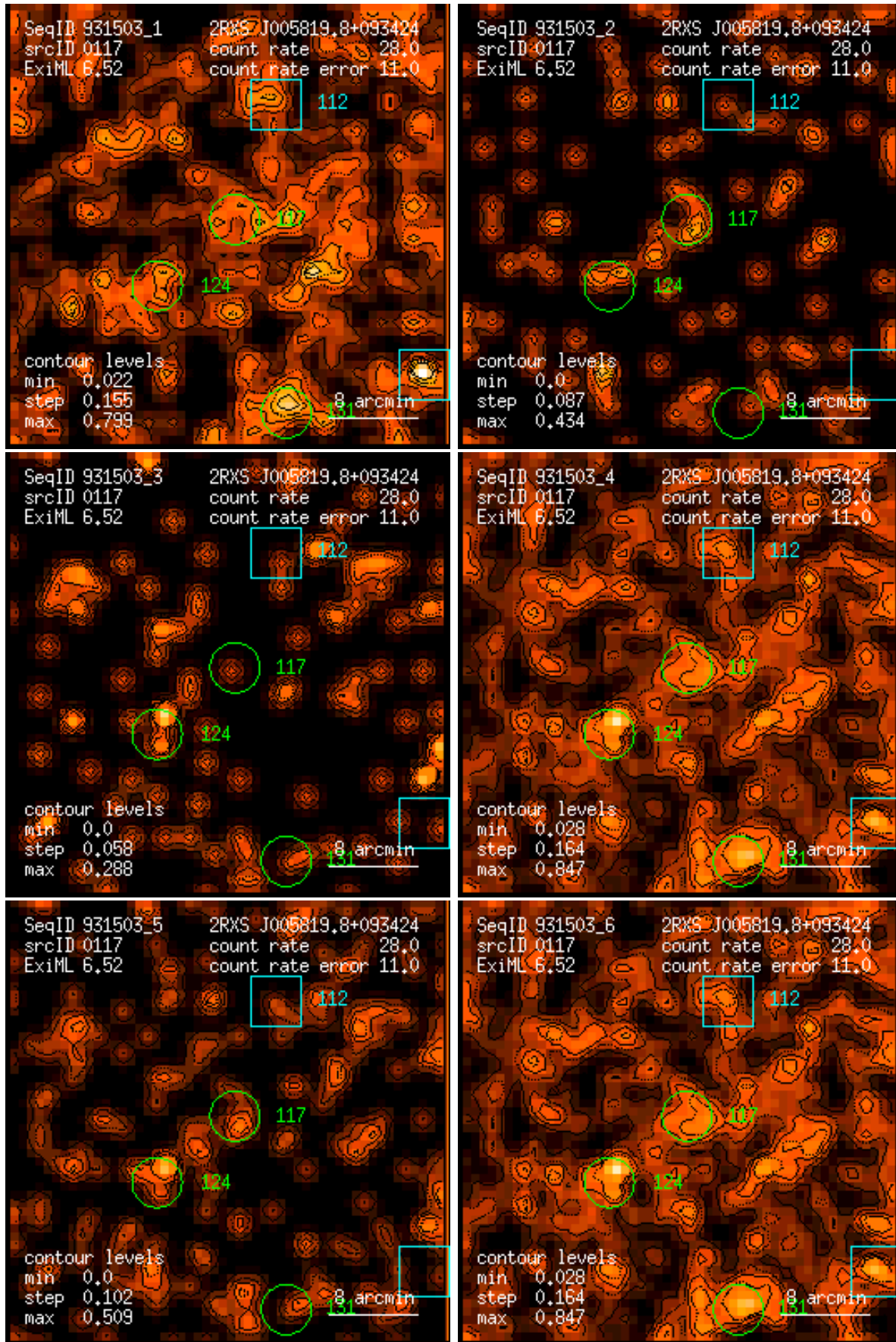
Figure 117: RASS 931503: detection 0117: band rate images, Gaussian filter: (1) PSPC channels 11 – 41, (2) 52 – 90, (3) 91 – 201, (4) 11 – 235, (5) 52 – 201, (6) 11 – 201. Broad band rates in counts/ks. Band rate contour levels in counts/ks/arcmin 2 .
