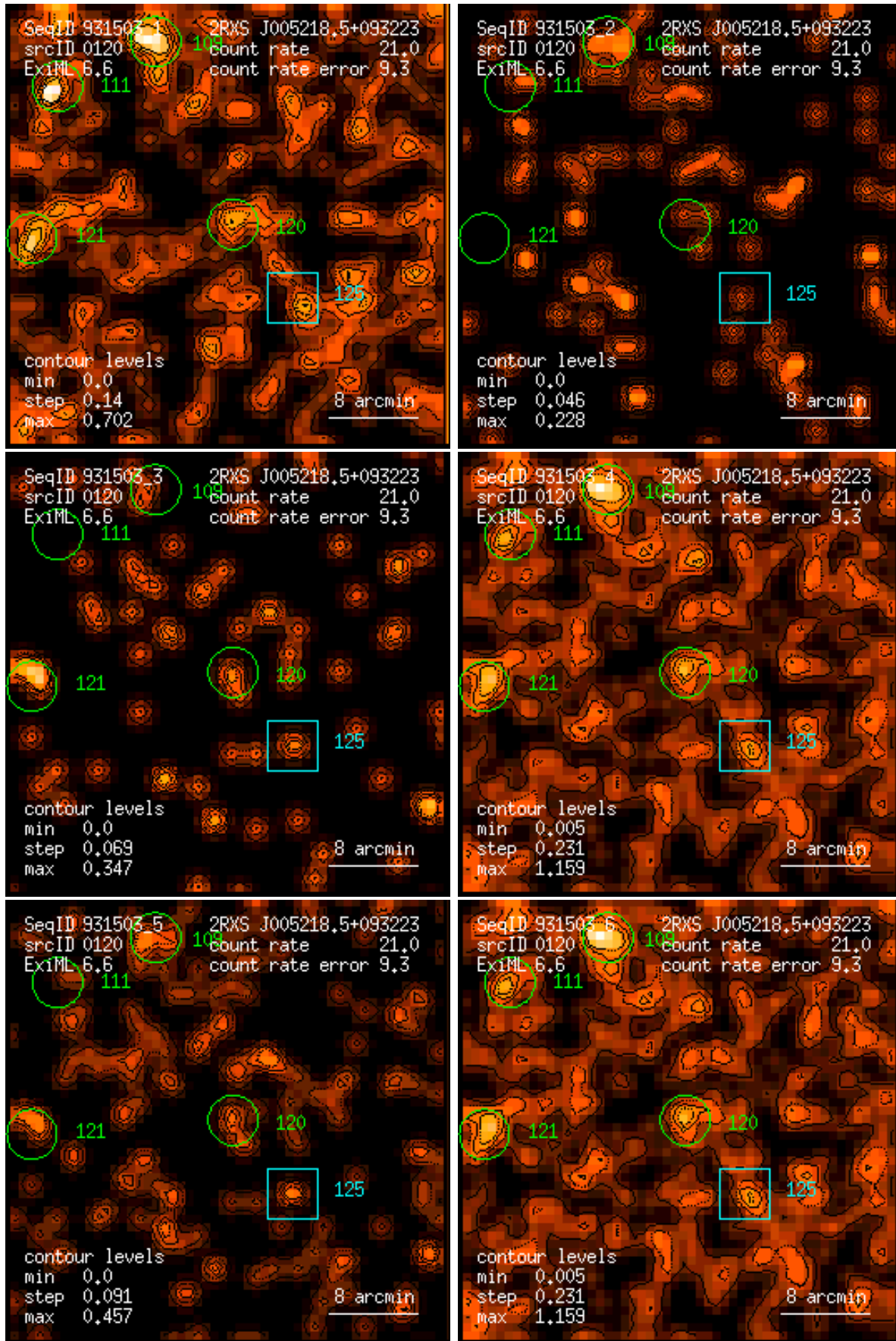
Figure 120: RASS 931503: detection 0120: band rate images, Gaussian filter: (1) PSPC channels 11 – 41, (2) 52 – 90, (3) 91 – 201, (4) 11 – 235, (5) 52 – 201, (6) 11 – 201. Broad band rates in counts/ks. Band rate contour levels in counts/ks/arcmin 2 .
