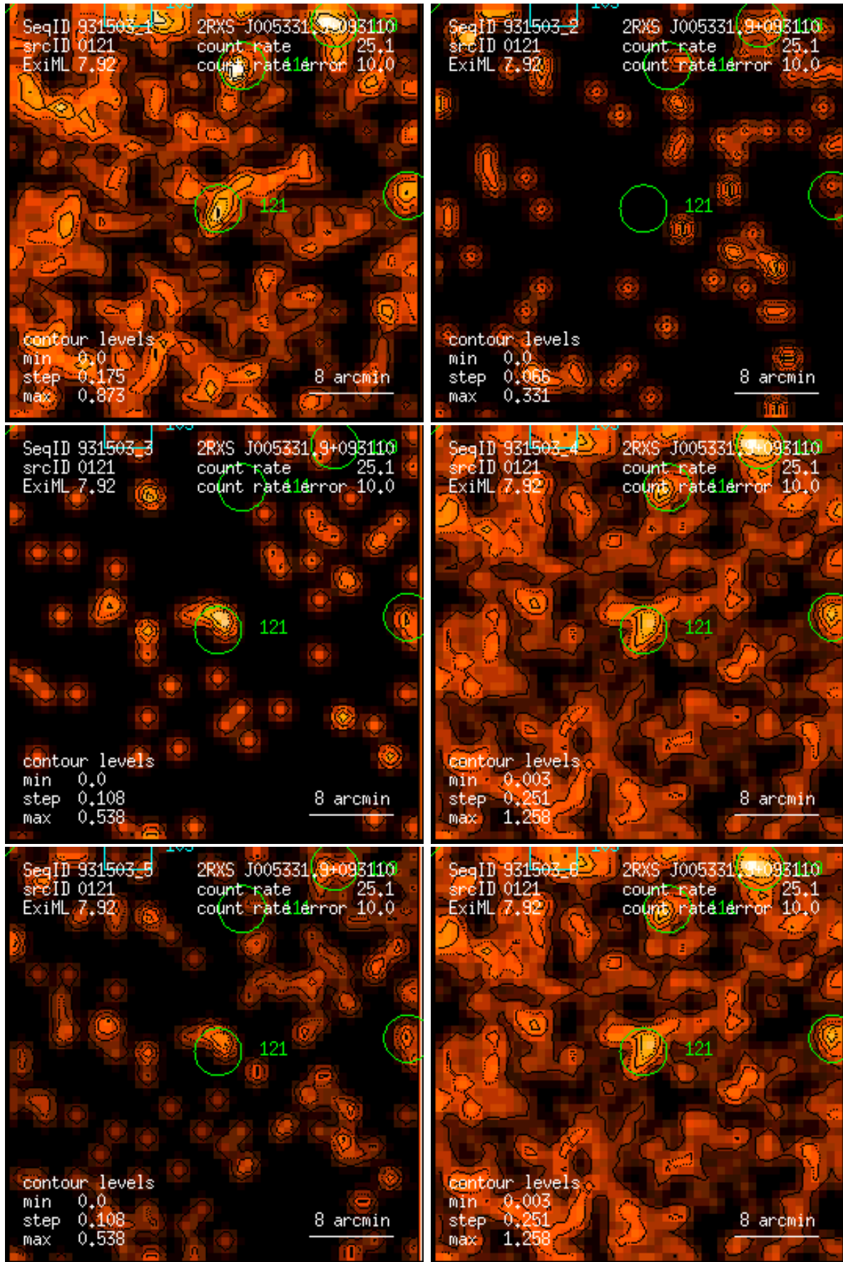
Figure 121: RASS 931503: detection 0121: band rate images, Gaussian filter: (1) PSPC channels 11 – 41, (2) 52 – 90, (3) 91 – 201, (4) 11 – 235, (5) 52 – 201, (6) 11 – 201. Broad band rates in counts/ks. Band rate contour levels in counts/ks/arcmin 2 .
