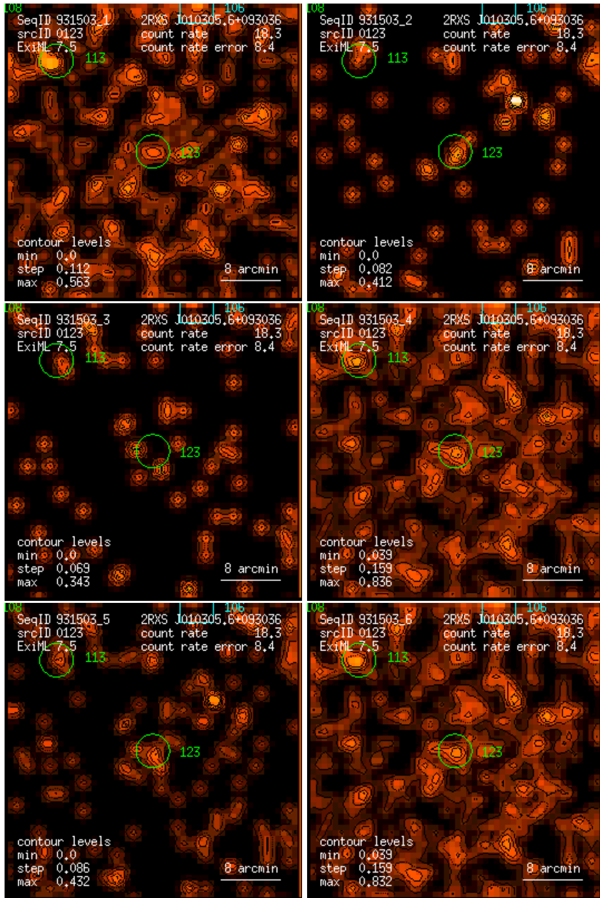
Figure 123: RASS 931503: detection 0123: band rate images, Gaussian filter: (1) PSPC channels 11 – 41, (2) 52 – 90, (3) 91 – 201, (4) 11 – 235, (5) 52 – 201, (6) 11 – 201. Broad band rates in counts/ks. Band rate contour levels in counts/ks/arcmin 2 .
