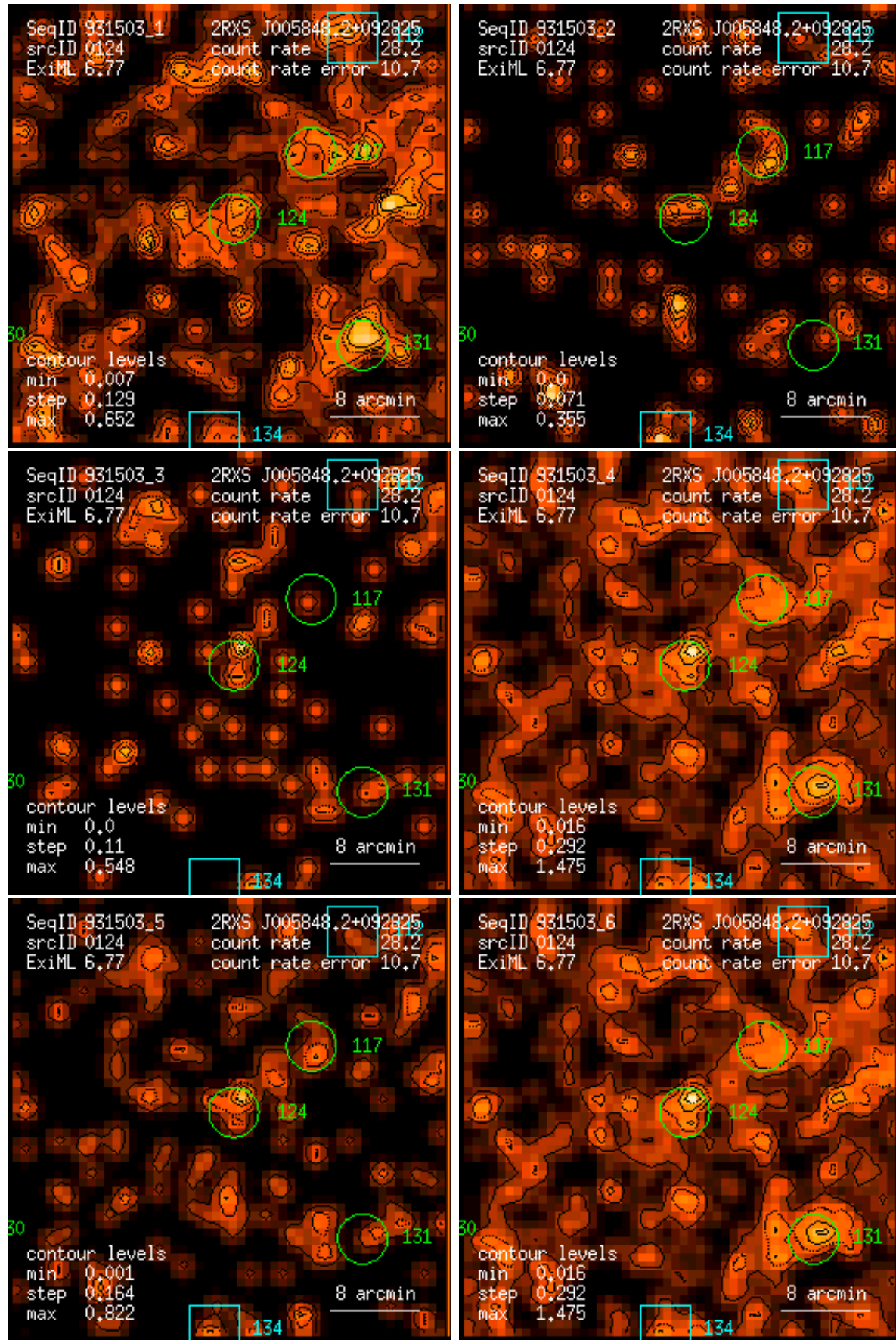
Figure 124: RASS 931503: detection 0124: band rate images, Gaussian filter: (1) PSPC channels 11 – 41, (2) 52 – 90, (3) 91 – 201, (4) 11 – 235, (5) 52 – 201, (6) 11 – 201. Broad band rates in counts/ks. Band rate contour levels in counts/ks/arcmin 2 .
