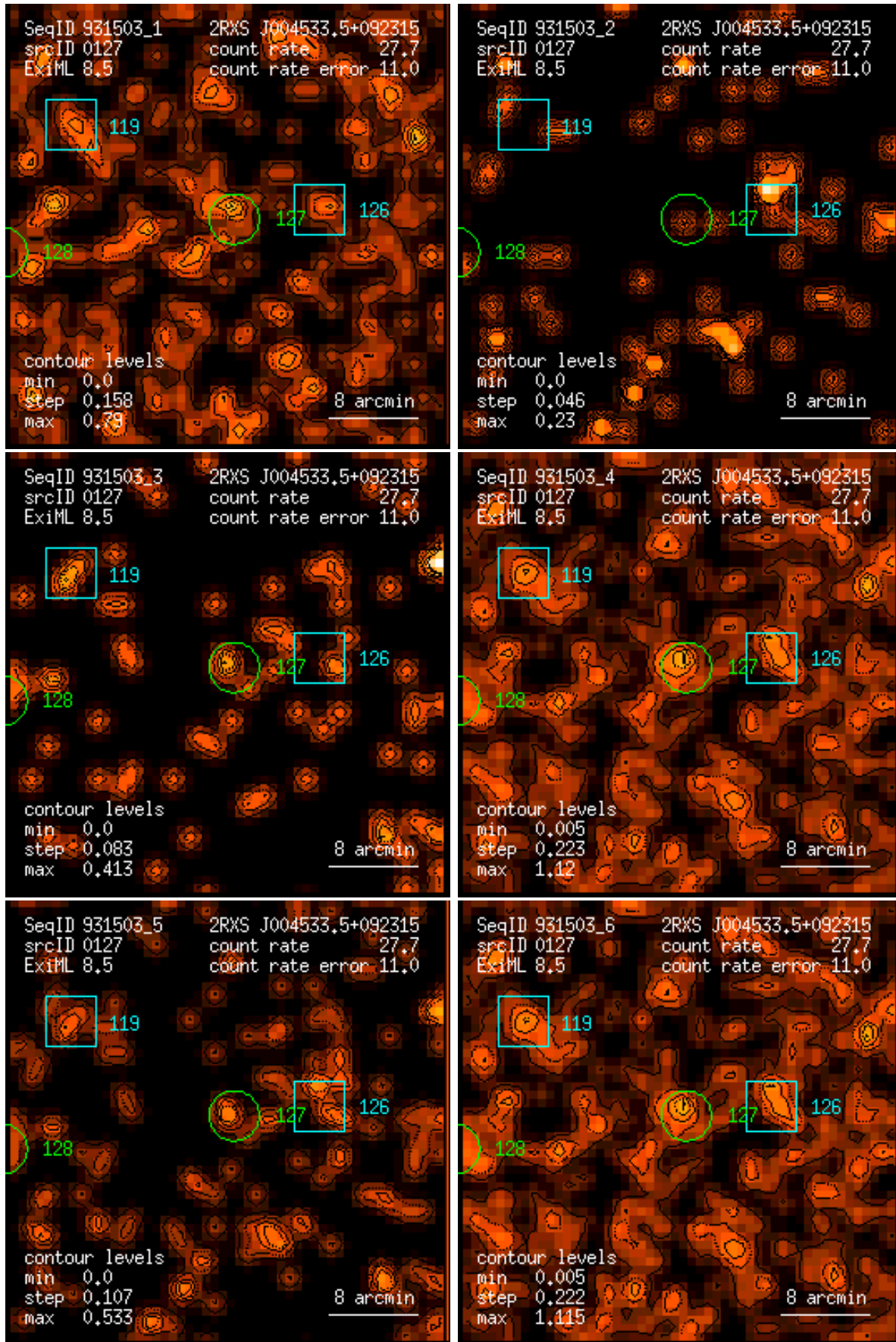
Figure 127: RASS 931503: detection 0127: band rate images, Gaussian filter: (1) PSPC channels 11 – 41, (2) 52 – 90, (3) 91 – 201, (4) 11 – 235, (5) 52 – 201, (6) 11 – 201. Broad band rates in counts/ks. Band rate contour levels in counts/ks/arcmin 2 .
