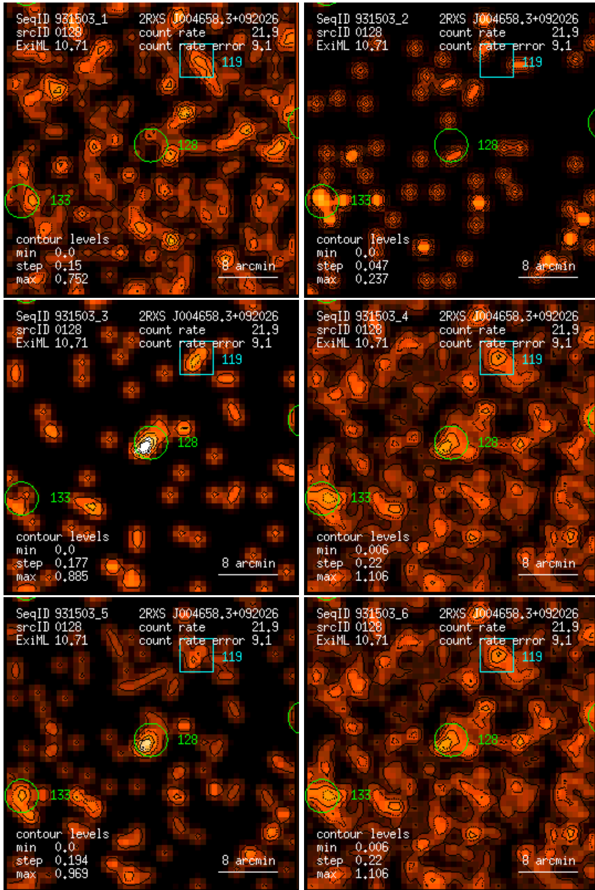
Figure 128: RASS 931503: detection 0128: band rate images, Gaussian filter: (1) PSPC channels 11 – 41, (2) 52 – 90, (3) 91 – 201, (4) 11 – 235, (5) 52 – 201, (6) 11 – 201. Broad band rates in counts/ks. Band rate contour levels in counts/ks/arcmin 2 .
