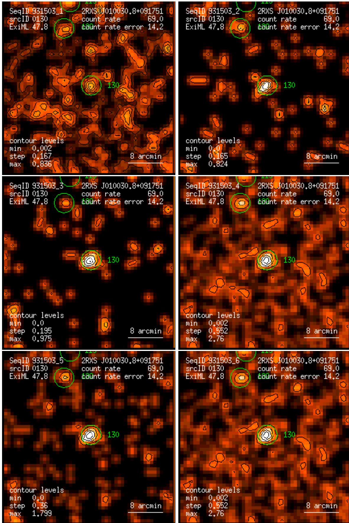
Figure 130: RASS 931503: detection 0130: band rate images, Gaussian filter: (1) PSPC channels 11 – 41, (2) 52 – 90, (3) 91 – 201, (4) 11 – 235, (5) 52 – 201, (6) 11 – 201. Broad band rates in counts/ks. Band rate contour levels in counts/ks/arcmin 2 .
