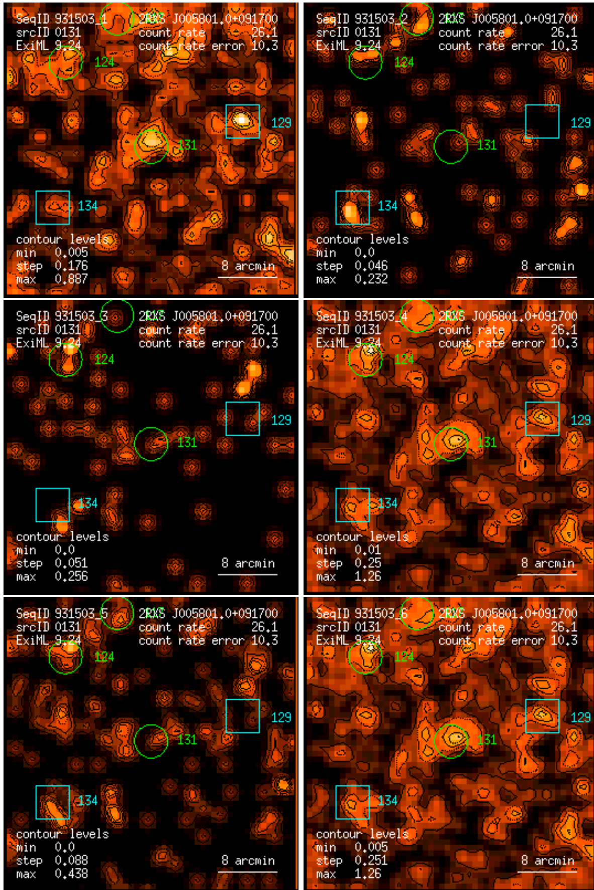
Figure 131: RASS 931503: detection 0131: band rate images, Gaussian filter: (1) PSPC channels 11 – 41, (2) 52 – 90, (3) 91 – 201, (4) 11 – 235, (5) 52 – 201, (6) 11 – 201. Broad band rates in counts/ks. Band rate contour levels in counts/ks/arcmin 2 .
