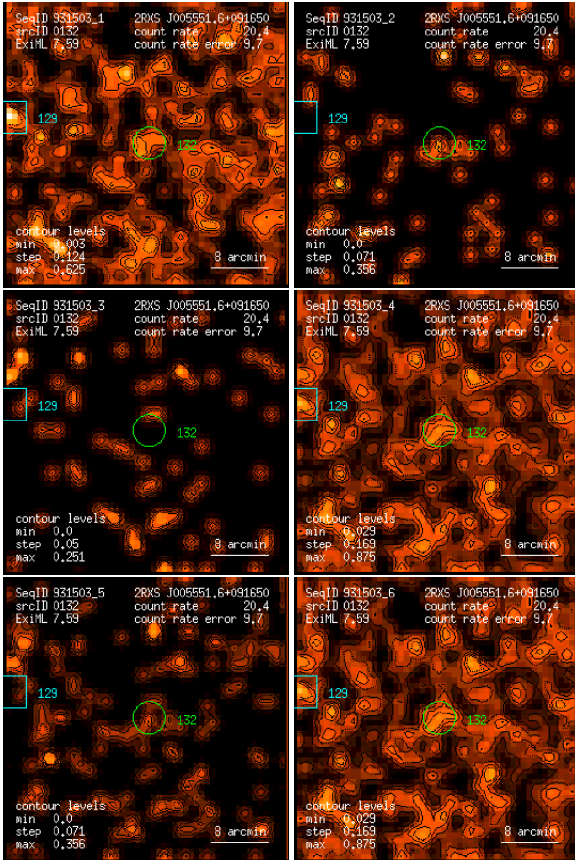
Figure 132: RASS 931503: detection 0132: band rate images, Gaussian filter: (1) PSPC channels 11 – 41, (2) 52 – 90, (3) 91 – 201, (4) 11 – 235, (5) 52 – 201, (6) 11 – 201. Broad band rates in counts/ks. Band rate contour levels in counts/ks/arcmin 2 .
