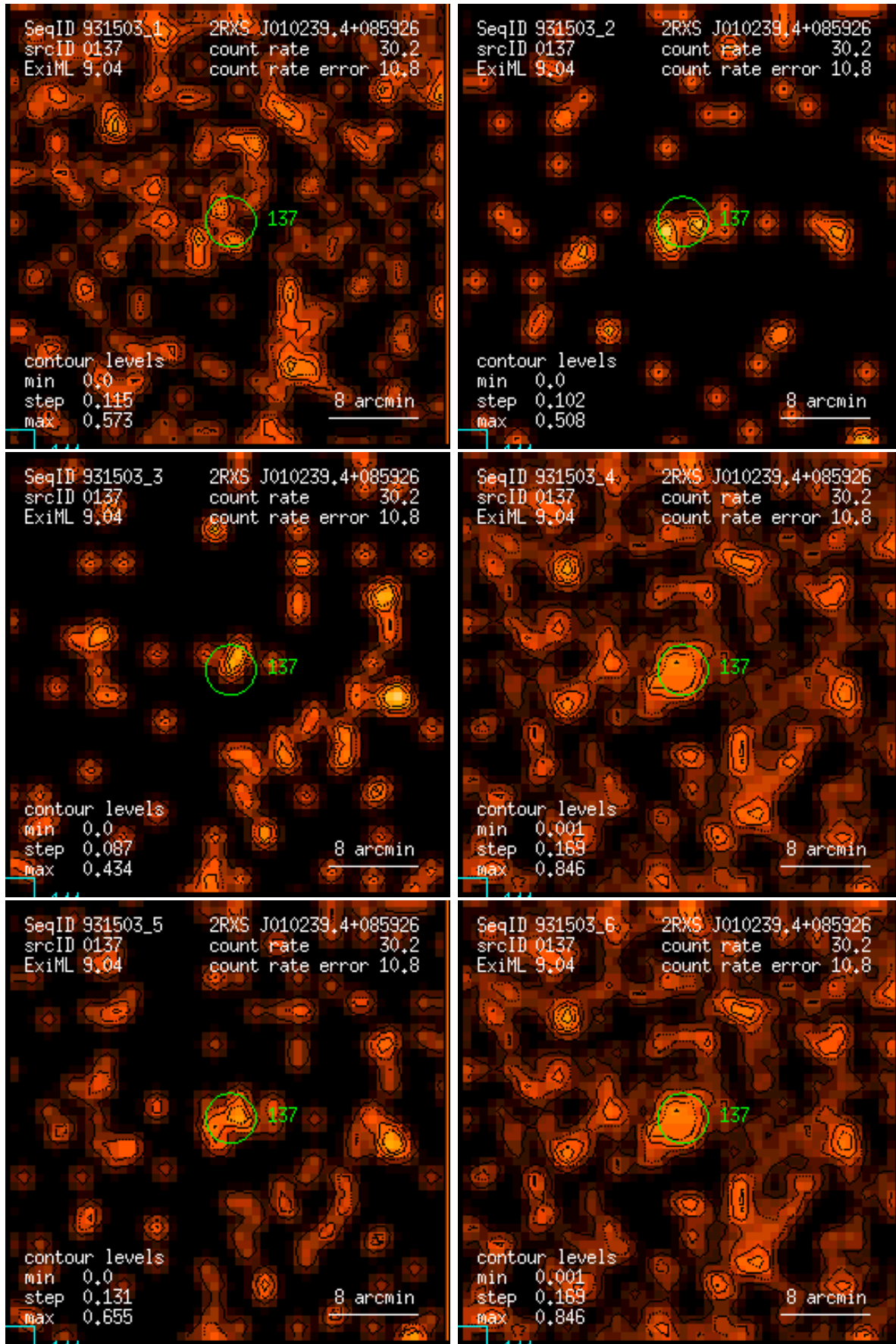
Figure 137: RASS 931503: detection 0137: band rate images, Gaussian filter: (1) PSPC channels 11 – 41, (2) 52 – 90, (3) 91 – 201, (4) 11 – 235, (5) 52 – 201, (6) 11 – 201. Broad band rates in counts/ks. Band rate contour levels in counts/ks/arcmin 2 .
