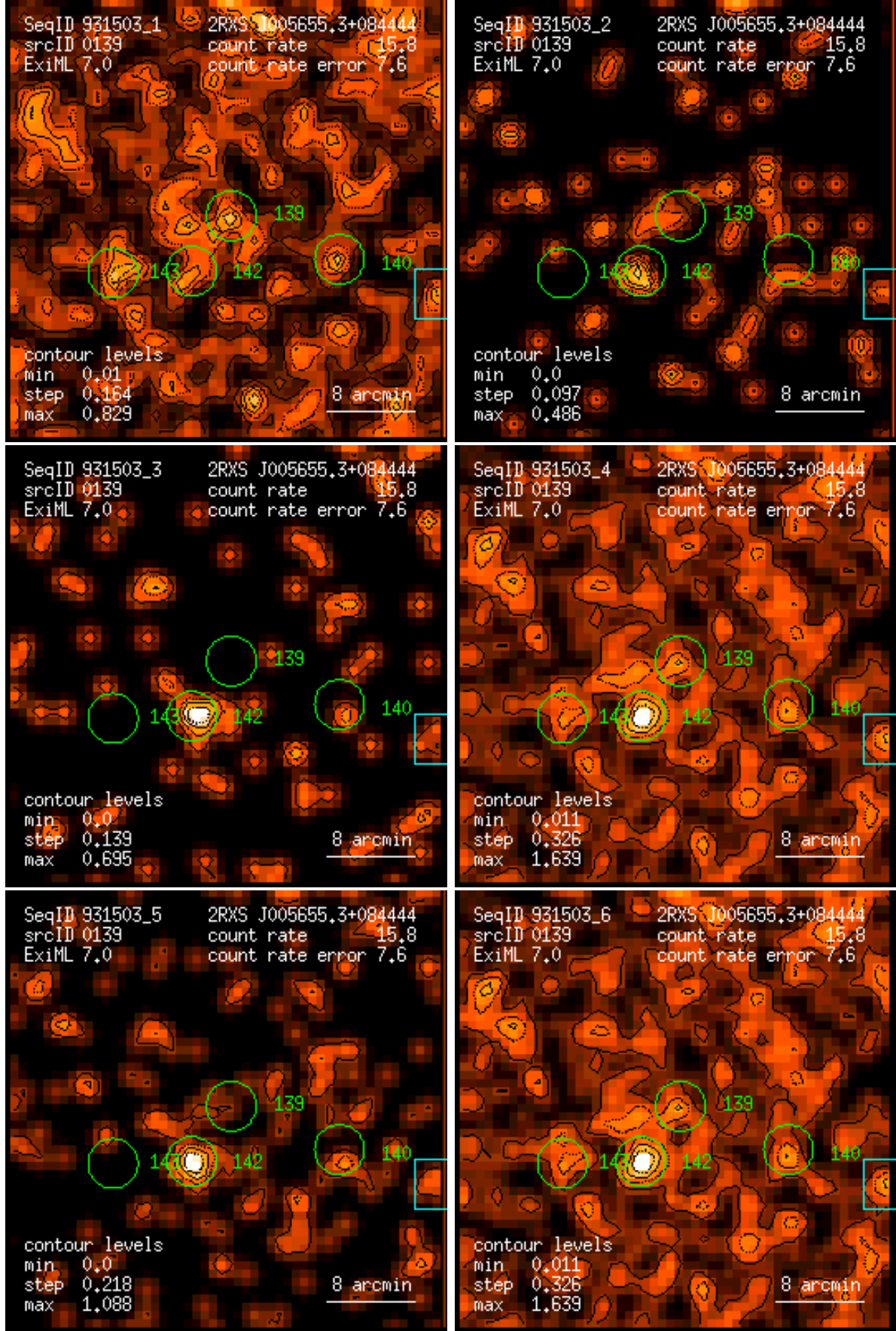
Figure 139: RASS 931503: detection 0139: band rate images, Gaussian filter: (1) PSPC channels 11 – 41, (2) 52 – 90, (3) 91 – 201, (4) 11 – 235, (5) 52 – 201, (6) 11 – 201. Broad band rates in counts/ks. Band rate contour levels in counts/ks/arcmin 2 .
