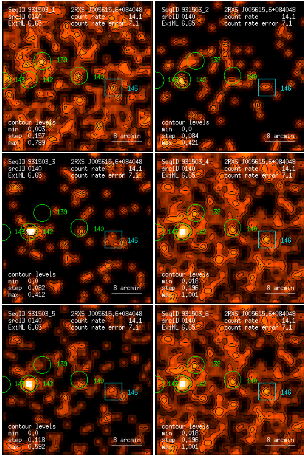
Figure 140: RASS 931503: detection 0140: band rate images, Gaussian filter: (1) PSPC channels 11 – 41, (2) 52 – 90, (3) 91 – 201, (4) 11 – 235, (5) 52 – 201, (6) 11 – 201. Broad band rates in counts/ks. Band rate contour levels in counts/ks/arcmin 2 .
