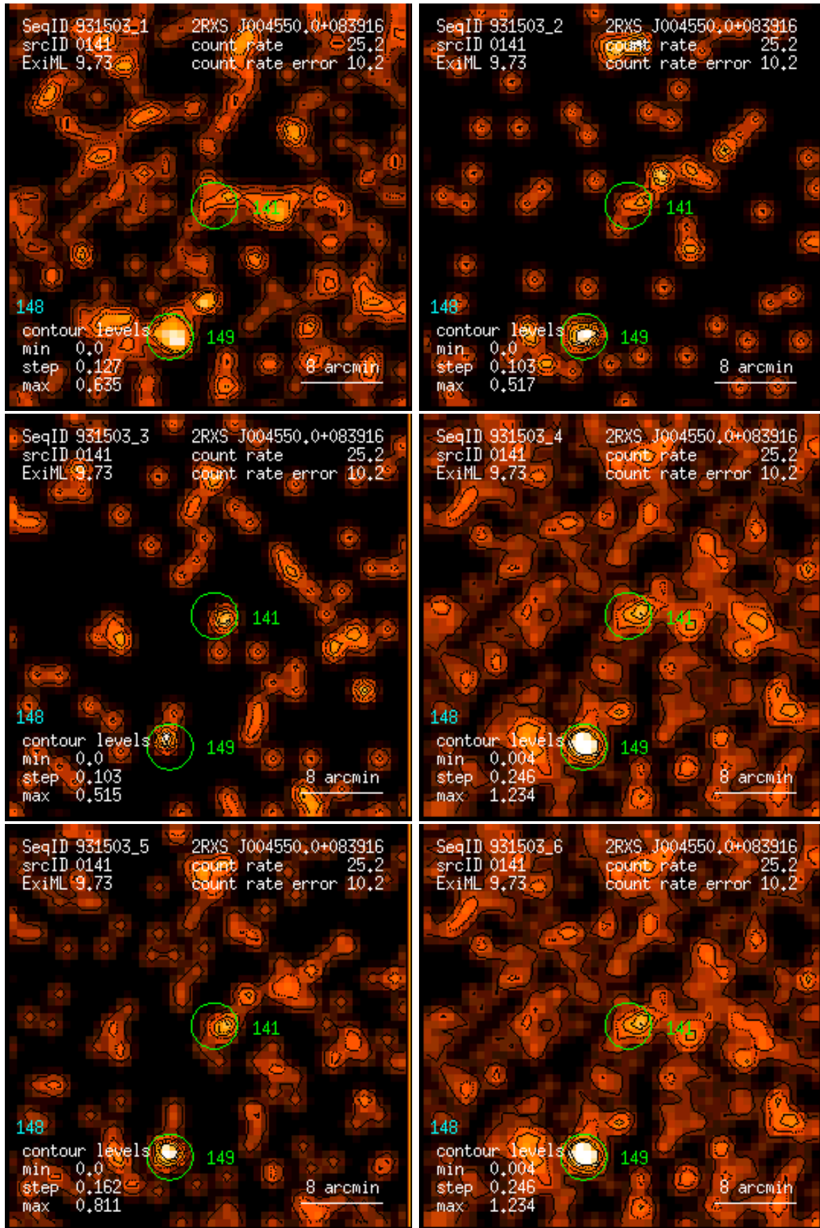
Figure 141: RASS 931503: detection 0141: band rate images, Gaussian filter: (1) PSPC channels 11 – 41, (2) 52 – 90, (3) 91 – 201, (4) 11 – 235, (5) 52 – 201, (6) 11 – 201. Broad band rates in counts/ks. Band rate contour levels in counts/ks/arcmin 2 .
