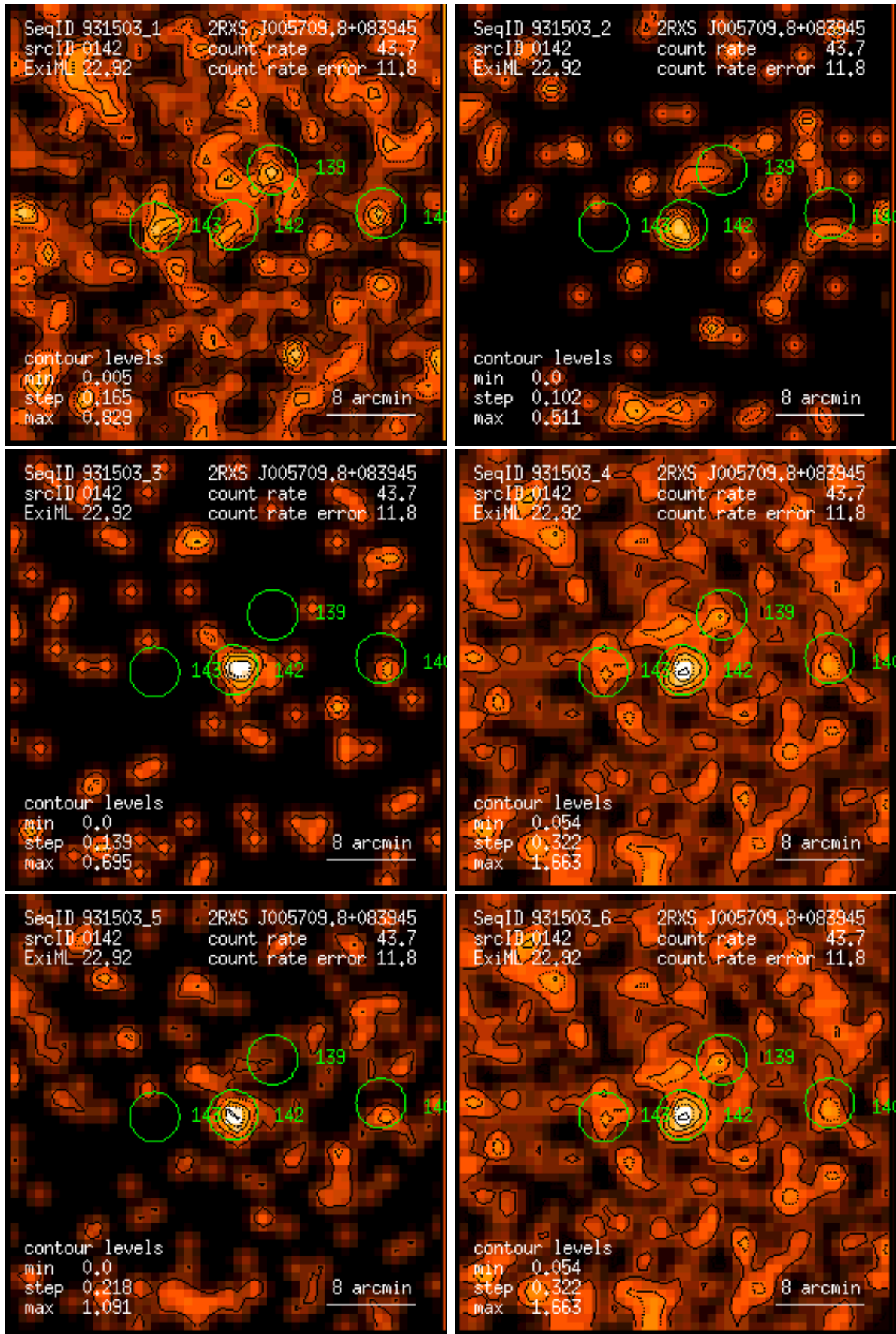
Figure 142: RASS 931503: detection 0142: band rate images, Gaussian filter: (1) PSPC channels 11 – 41, (2) 52 – 90, (3) 91 – 201, (4) 11 – 235, (5) 52 – 201, (6) 11 – 201. Broad band rates in counts/ks. Band rate contour levels in counts/ks/arcmin 2 .
