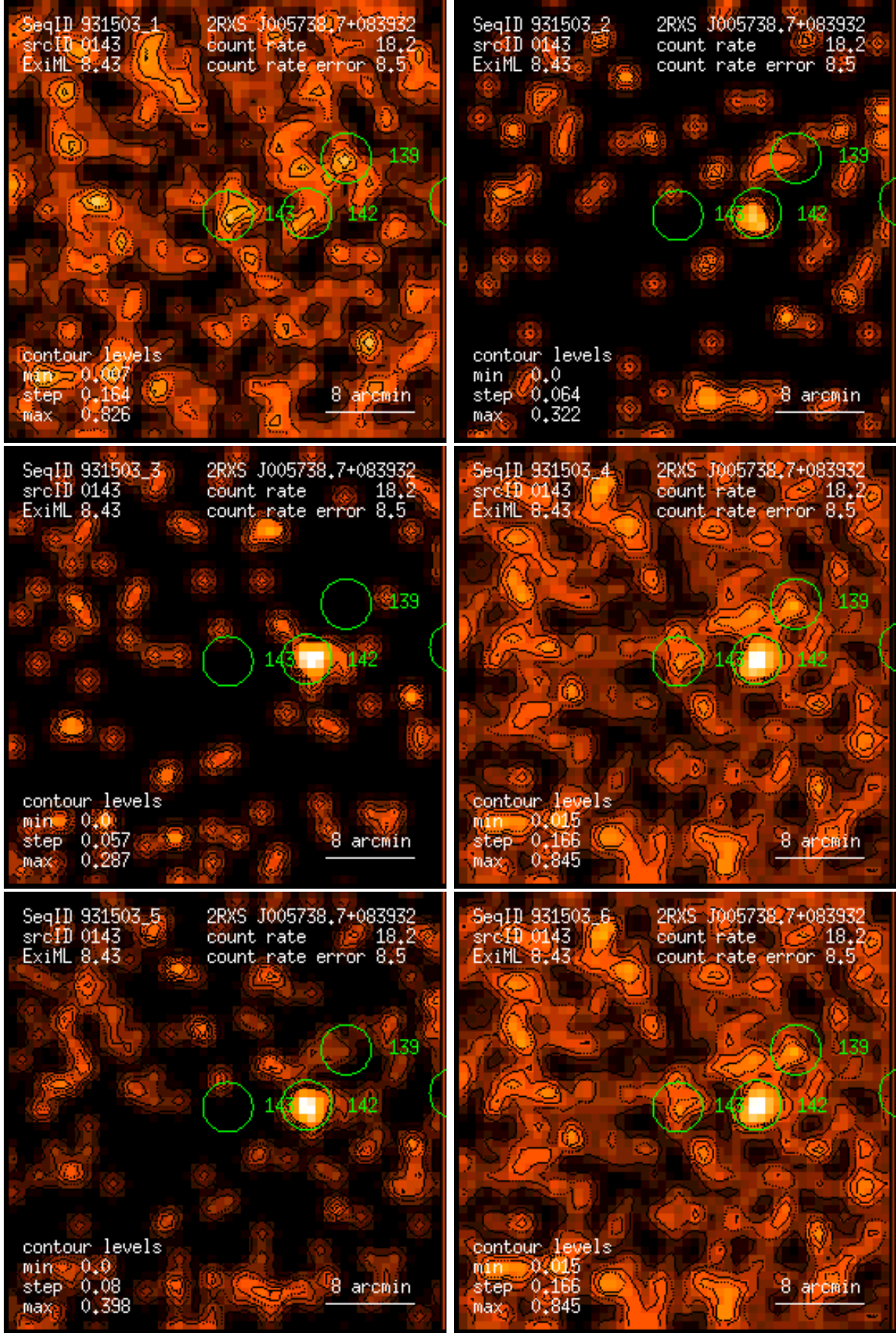
Figure 143: RASS 931503: detection 0143: band rate images, Gaussian filter: (1) PSPC channels 11 – 41, (2) 52 – 90, (3) 91 – 201, (4) 11 – 235, (5) 52 – 201, (6) 11 – 201. Broad band rates in counts/ks. Band rate contour levels in counts/ks/arcmin 2 .
