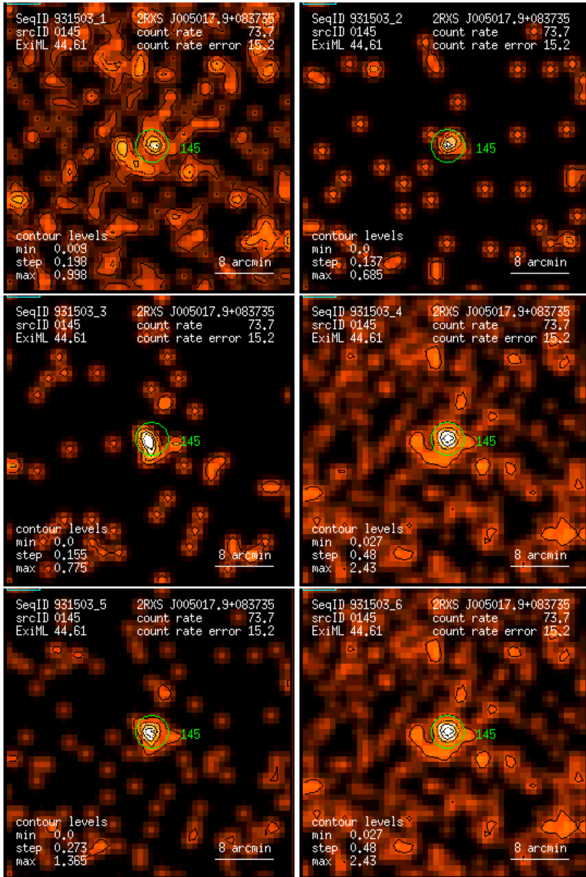
Figure 145: RASS 931503: detection 0145: band rate images, Gaussian filter: (1) PSPC channels 11 – 41, (2) 52 – 90, (3) 91 – 201, (4) 11 – 235, (5) 52 – 201, (6) 11 – 201. Broad band rates in counts/ks. Band rate contour levels in counts/ks/arcmin 2 .
