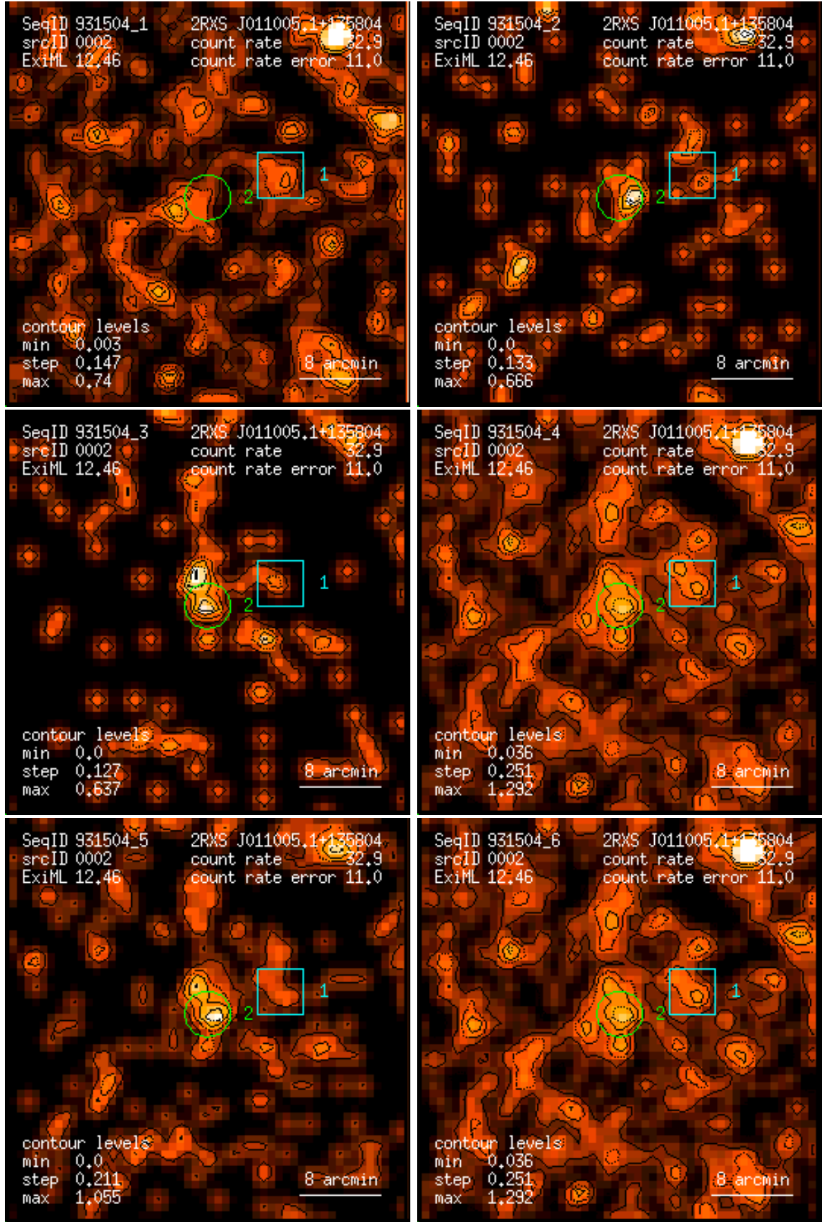
Figure 2: RASS 931504: detection 0002: band rate images, Gaussian filter: (1) PSPC channels 11 – 41, (2) 52 – 90, (3) 91 – 201, (4) 11 – 235, (5) 52 – 201, (6) 11 – 201. Broad band rates in counts/ks. Band rate contour levels in counts/ks/arcmin 2 .
