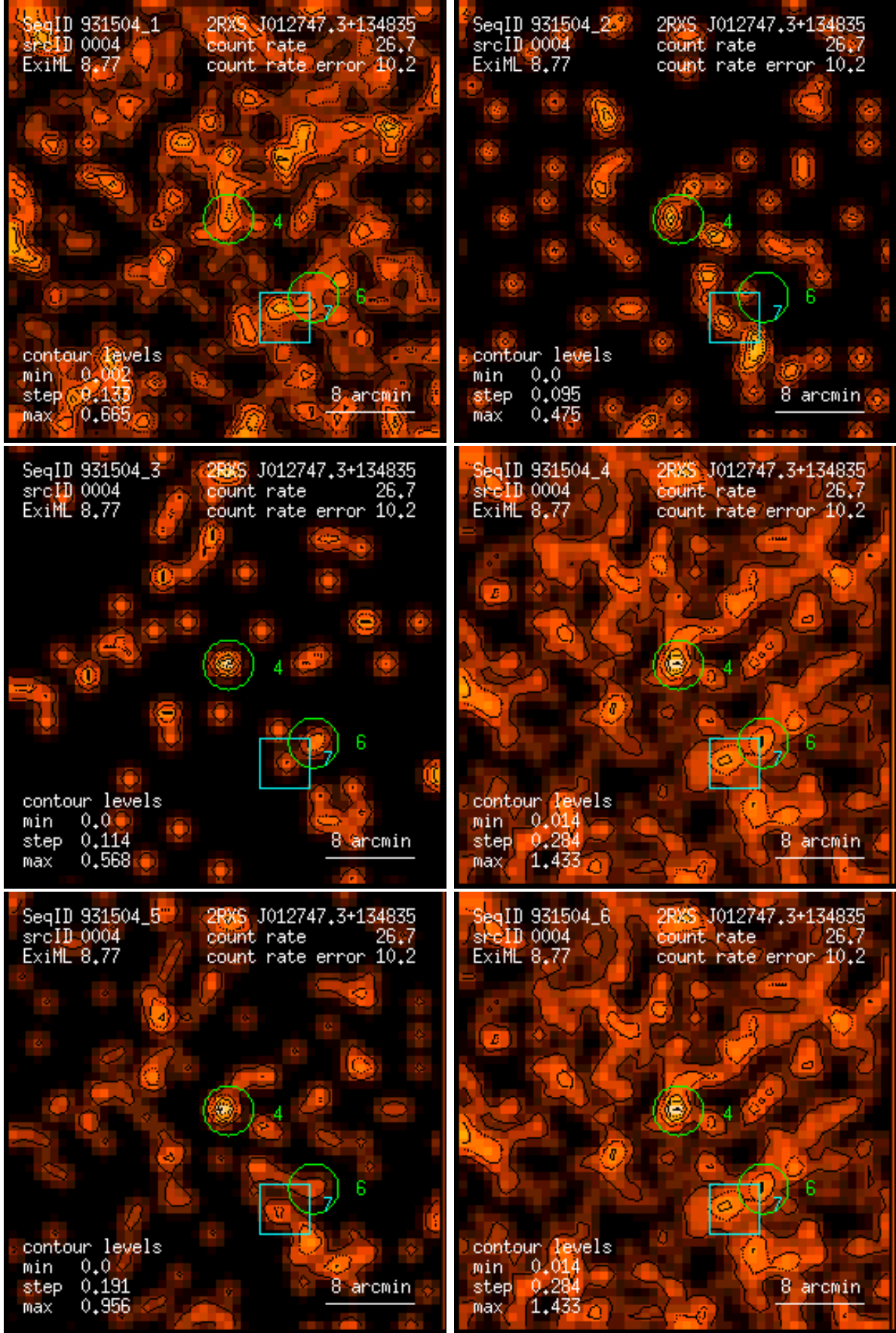
Figure 4: RASS 931504: detection 0004: band rate images, Gaussian filter: (1) PSPC channels 11 – 41, (2) 52 – 90, (3) 91 – 201, (4) 11 – 235, (5) 52 – 201, (6) 11 – 201. Broad band rates in counts/ks. Band rate contour levels in counts/ks/arcmin 2 .
