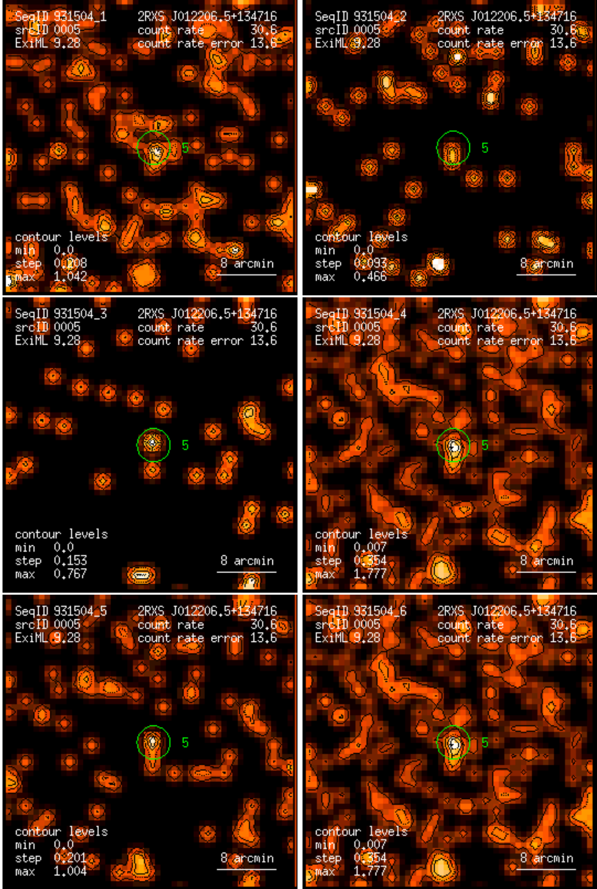
Figure 5: RASS 931504: detection 0005: band rate images, Gaussian filter: (1) PSPC channels 11 – 41, (2) 52 – 90, (3) 91 – 201, (4) 11 – 235, (5) 52 – 201, (6) 11 – 201. Broad band rates in counts/ks. Band rate contour levels in counts/ks/arcmin 2 .
