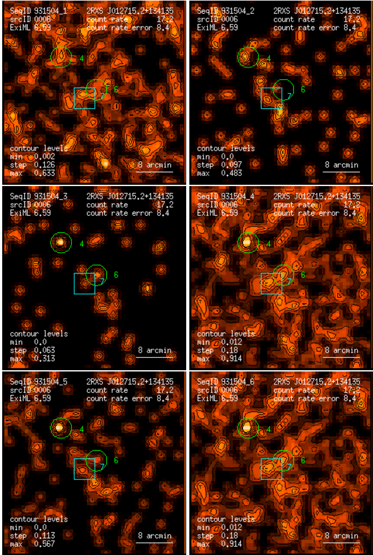
Figure 6: RASS 931504: detection 0006: band rate images, Gaussian filter: (1) PSPC channels 11 – 41, (2) 52 – 90, (3) 91 – 201, (4) 11 – 235, (5) 52 – 201, (6) 11 – 201. Broad band rates in counts/ks. Band rate contour levels in counts/ks/arcmin 2 .
