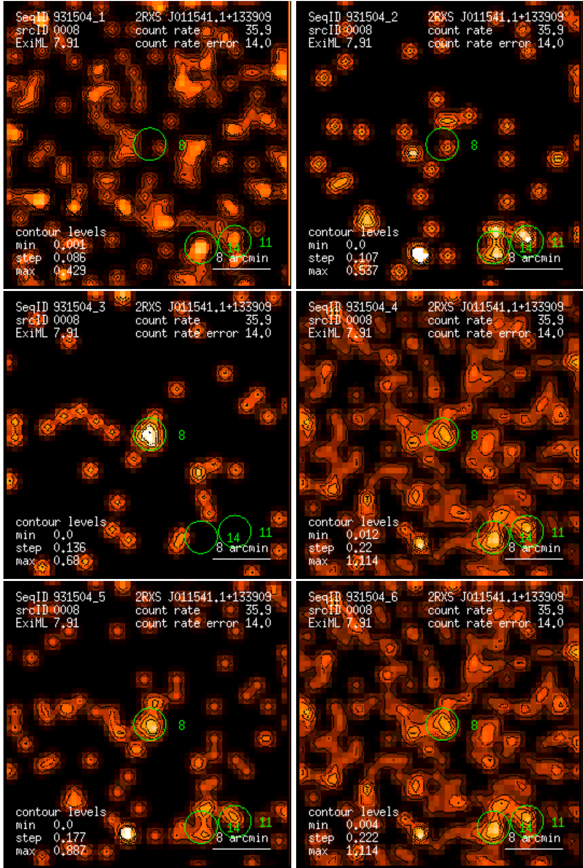
Figure 8: RASS 931504: detection 0008: band rate images, Gaussian filter: (1) PSPC channels 11 – 41, (2) 52 – 90, (3) 91 – 201, (4) 11 – 235, (5) 52 – 201, (6) 11 – 201. Broad band rates in counts/ks. Band rate contour levels in counts/ks/arcmin 2 .
