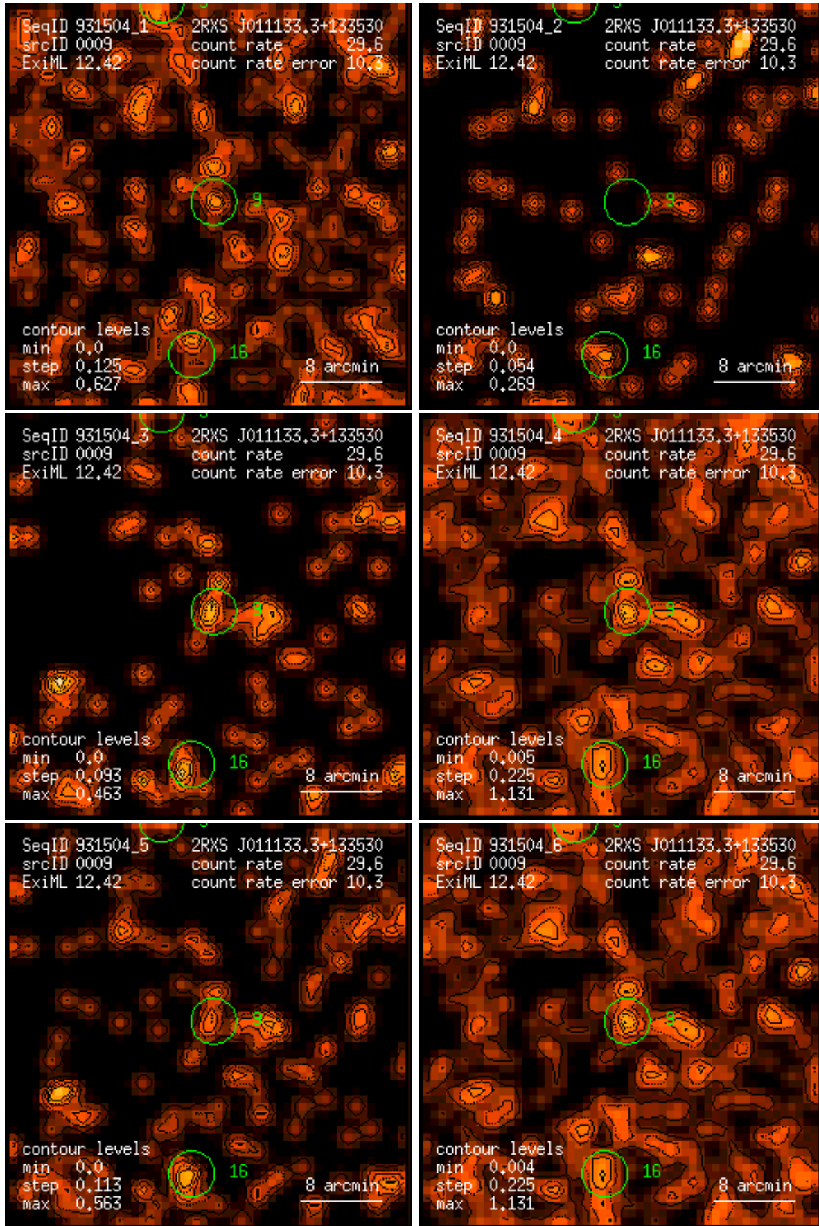
Figure 9: RASS 931504: detection 0009: band rate images, Gaussian filter: (1) PSPC channels 11 – 41, (2) 52 – 90, (3) 91 – 201, (4) 11 – 235, (5) 52 – 201, (6) 11 – 201. Broad band rates in counts/ks. Band rate contour levels in counts/ks/arcmin 2 .
