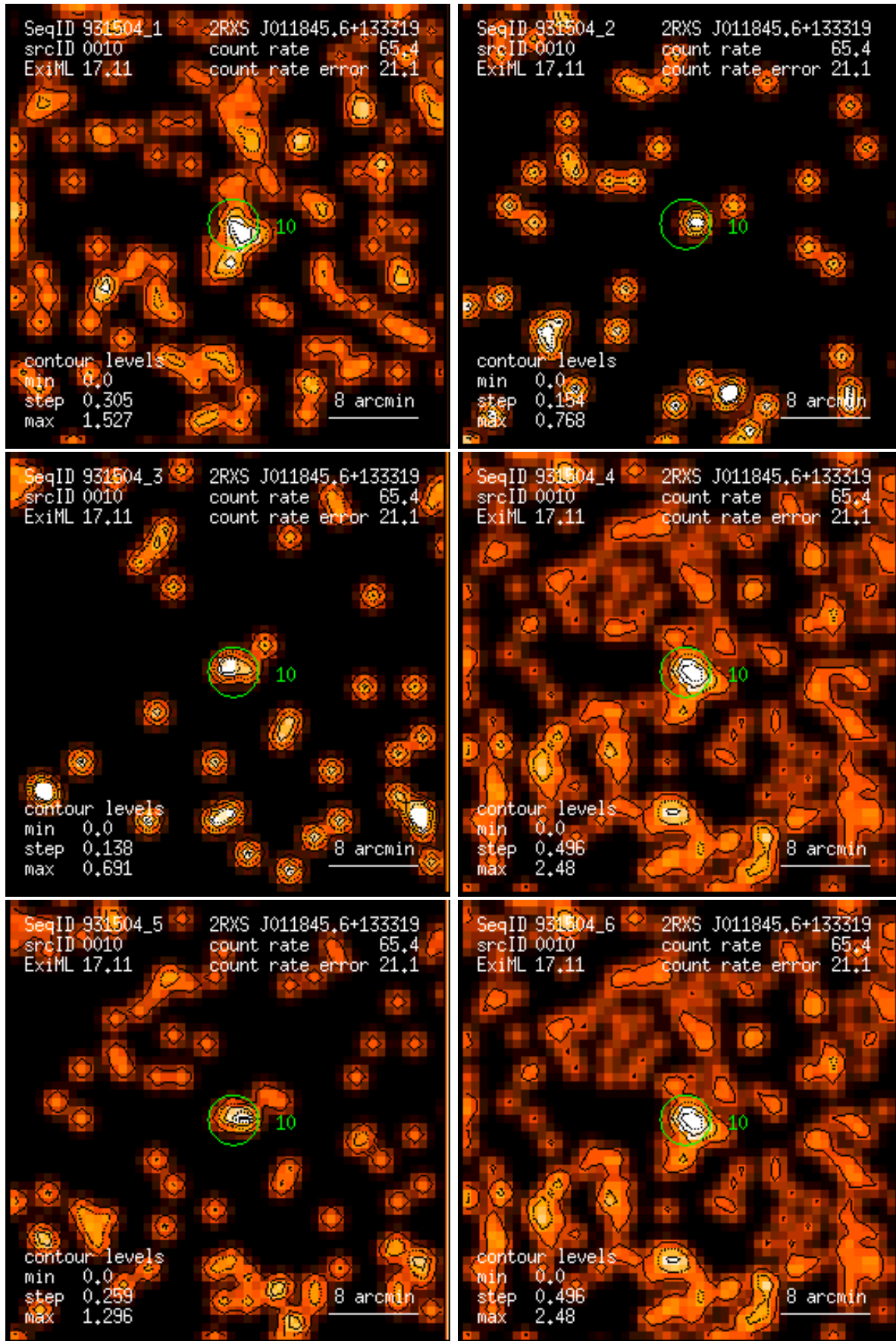
Figure 10: RASS 931504: detection 0010: band rate images, Gaussian filter: (1) PSPC channels 11 – 41, (2) 52 – 90, (3) 91 – 201, (4) 11 – 235, (5) 52 – 201, (6) 11 – 201. Broad band rates in counts/ks. Band rate contour levels in counts/ks/arcmin 2 .
