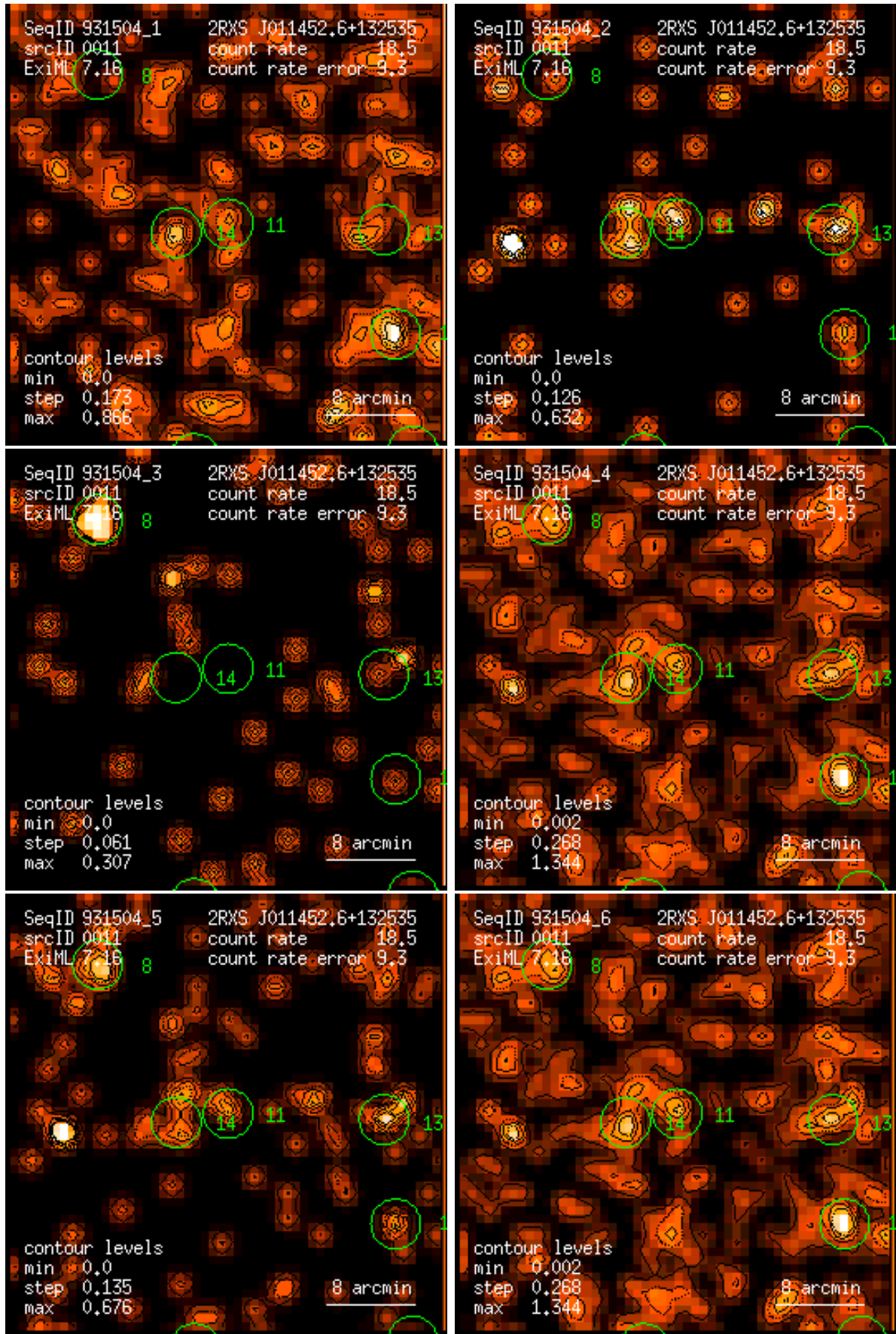
Figure 11: RASS 931504: detection 0011: band rate images, Gaussian filter: (1) PSPC channels 11 – 41, (2) 52 – 90, (3) 91 – 201, (4) 11 – 235, (5) 52 – 201, (6) 11 – 201. Broad band rates in counts/ks. Band rate contour levels in counts/ks/arcmin 2 .
