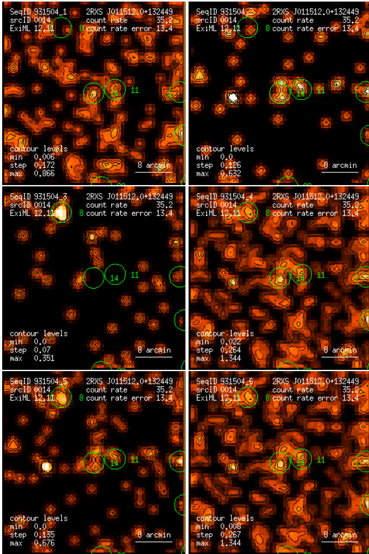
Figure 14: RASS 931504: detection 0014: band rate images, Gaussian filter: (1) PSPC channels 11 – 41, (2) 52 – 90, (3) 91 – 201, (4) 11 – 235, (5) 52 – 201, (6) 11 – 201. Broad band rates in counts/ks. Band rate contour levels in counts/ks/arcmin 2 .
