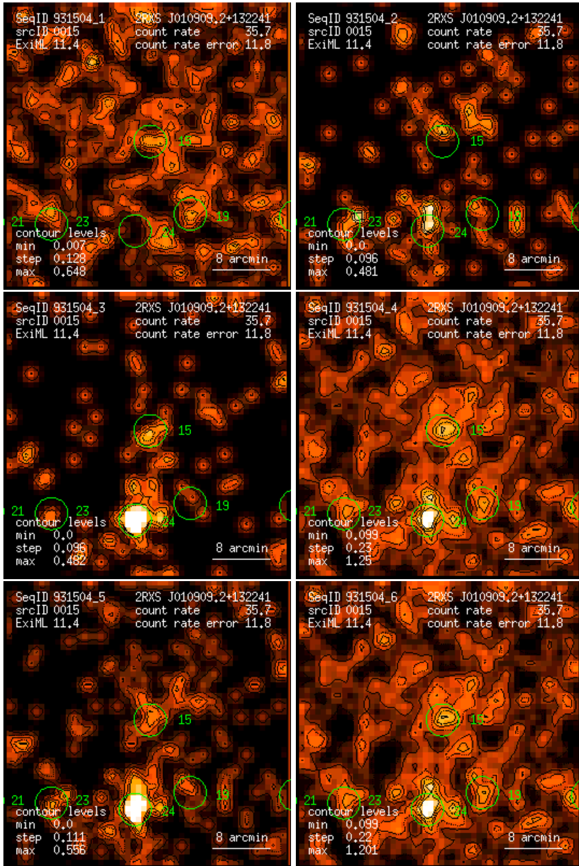
Figure 15: RASS 931504: detection 0015: band rate images, Gaussian filter: (1) PSPC channels 11 – 41, (2) 52 – 90, (3) 91 – 201, (4) 11 – 235, (5) 52 – 201, (6) 11 – 201. Broad band rates in counts/ks. Band rate contour levels in counts/ks/arcmin 2 .
