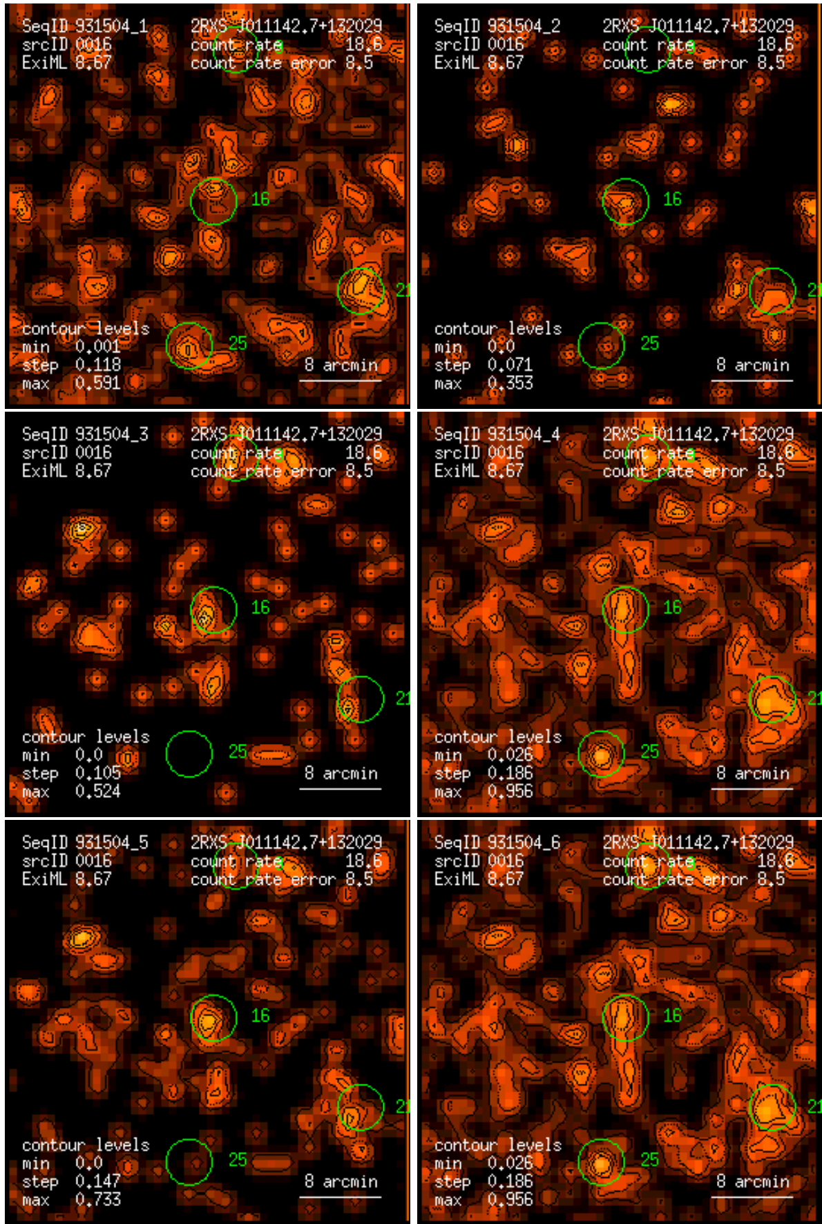
Figure 16: RASS 931504: detection 0016: band rate images, Gaussian filter: (1) PSPC channels 11 – 41, (2) 52 – 90, (3) 91 – 201, (4) 11 – 235, (5) 52 – 201, (6) 11 – 201. Broad band rates in counts/ks. Band rate contour levels in counts/ks/arcmin 2 .
