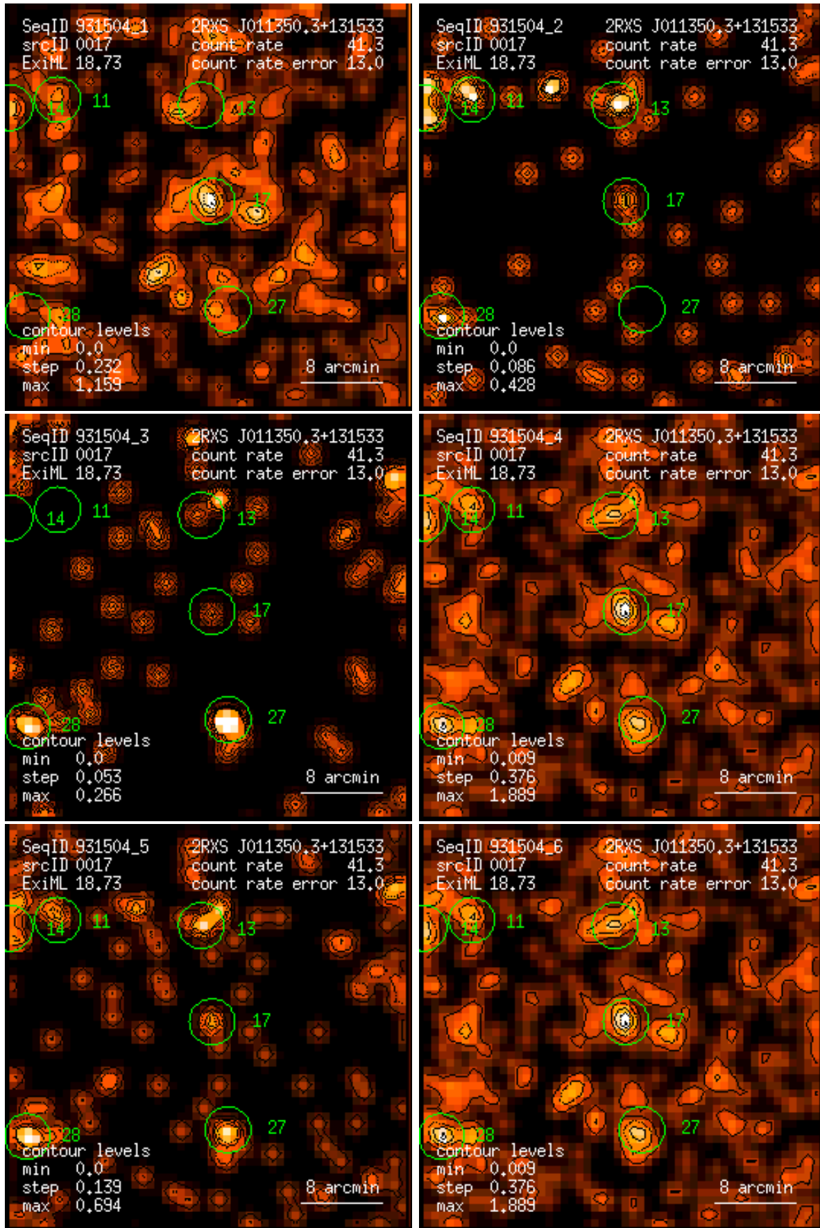
Figure 17: RASS 931504: detection 0017: band rate images, Gaussian filter: (1) PSPC channels 11 – 41, (2) 52 – 90, (3) 91 – 201, (4) 11 – 235, (5) 52 – 201, (6) 11 – 201. Broad band rates in counts/ks. Band rate contour levels in counts/ks/arcmin 2 .
