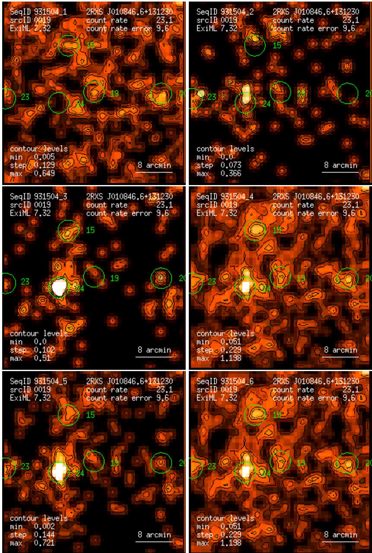
Figure 19: RASS 931504: detection 0019: band rate images, Gaussian filter: (1) PSPC channels 11 – 41, (2) 52 – 90, (3) 91 – 201, (4) 11 – 235, (5) 52 – 201, (6) 11 – 201. Broad band rates in counts/ks. Band rate contour levels in counts/ks/arcmin 2 .
