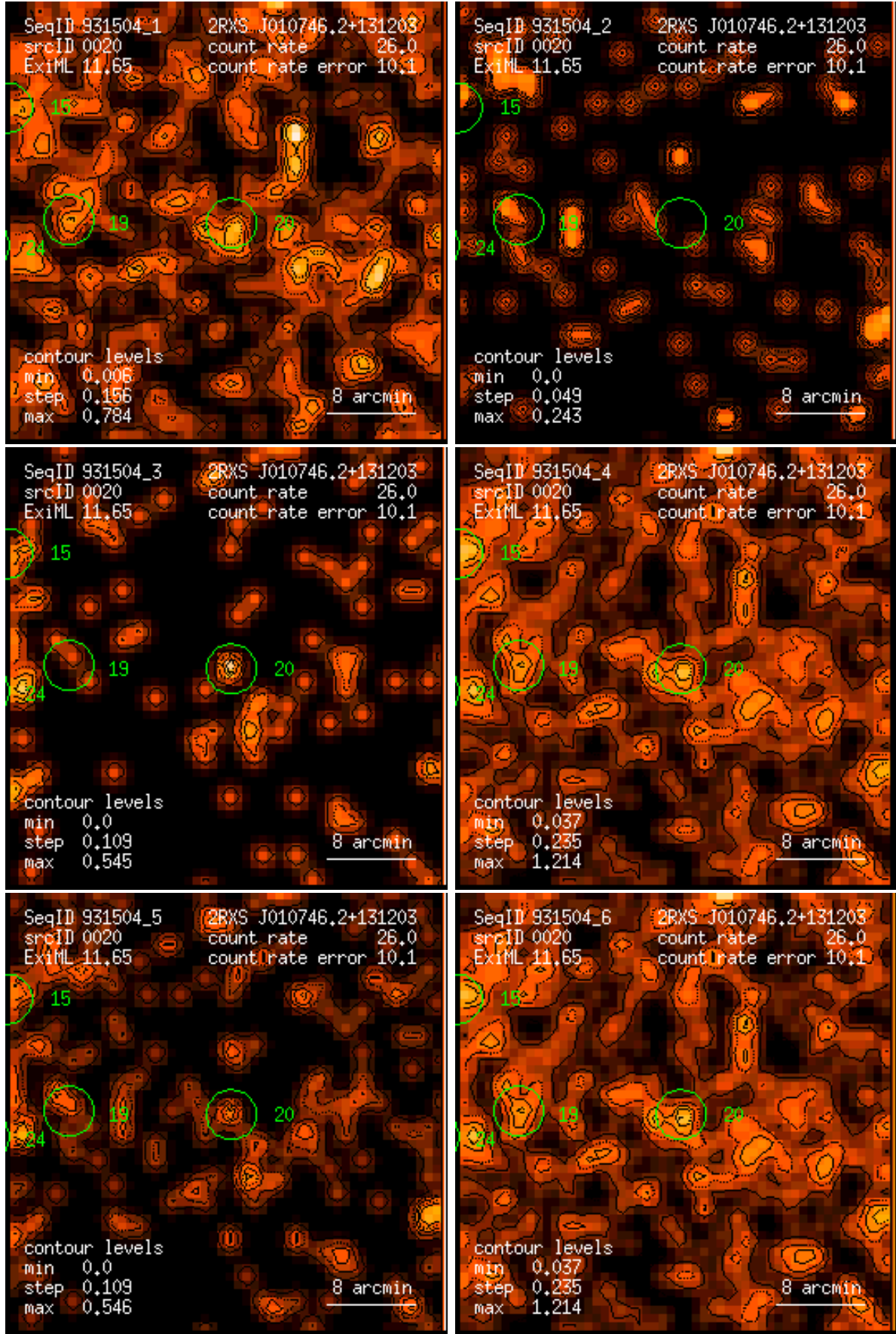
Figure 20: RASS 931504: detection 0020: band rate images, Gaussian filter: (1) PSPC channels 11 – 41, (2) 52 – 90, (3) 91 – 201, (4) 11 – 235, (5) 52 – 201, (6) 11 – 201. Broad band rates in counts/ks. Band rate contour levels in counts/ks/arcmin 2 .
