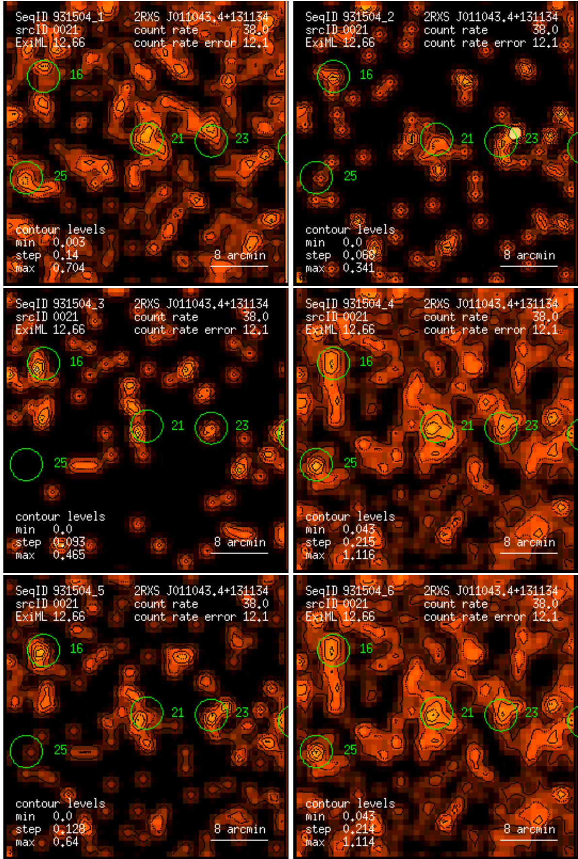
Figure 21: RASS 931504: detection 0021: band rate images, Gaussian filter: (1) PSPC channels 11 – 41, (2) 52 – 90, (3) 91 – 201, (4) 11 – 235, (5) 52 – 201, (6) 11 – 201. Broad band rates in counts/ks. Band rate contour levels in counts/ks/arcmin 2 .
