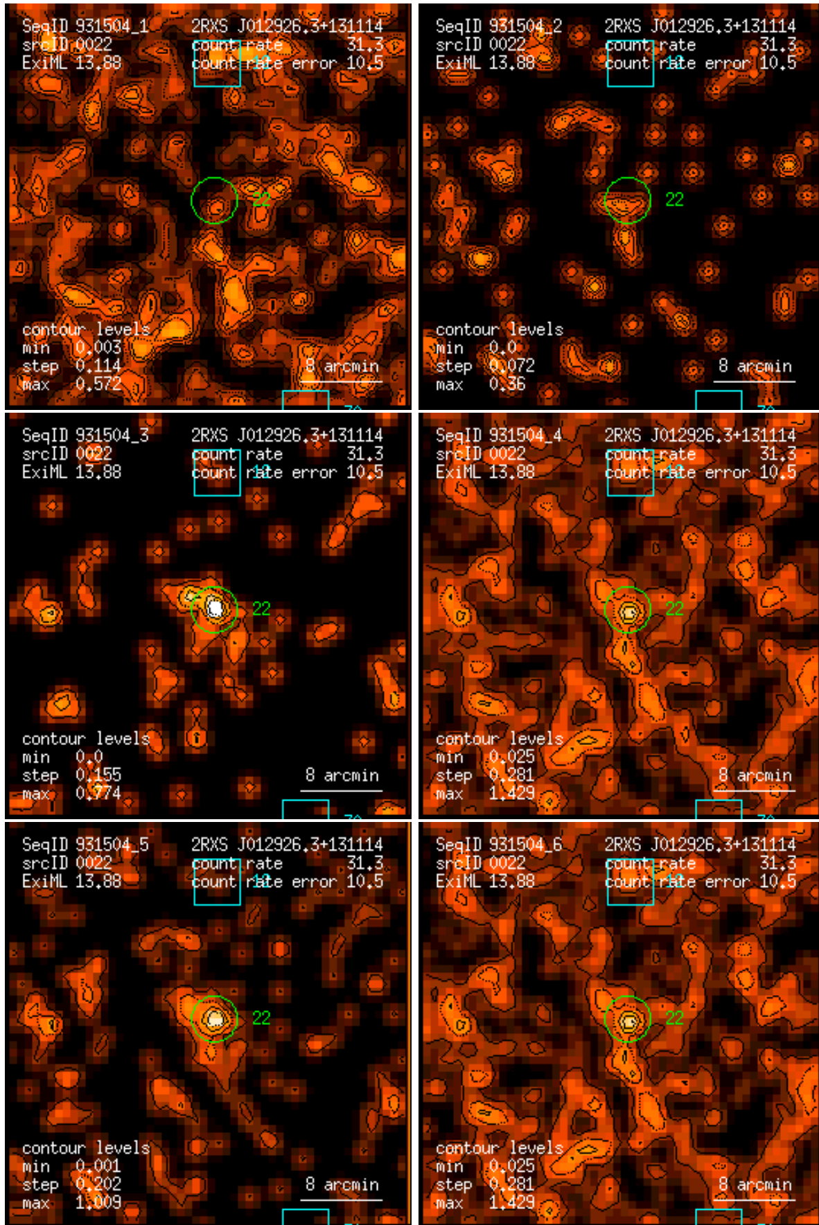
Figure 22: RASS 931504: detection 0022: band rate images, Gaussian filter: (1) PSPC channels 11 – 41, (2) 52 – 90, (3) 91 – 201, (4) 11 – 235, (5) 52 – 201, (6) 11 – 201. Broad band rates in counts/ks. Band rate contour levels in counts/ks/arcmin 2 .
