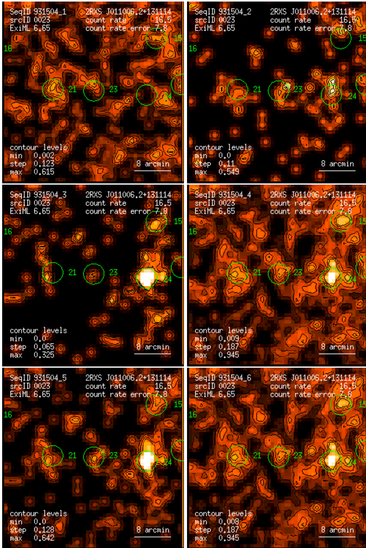
Figure 23: RASS 931504: detection 0023: band rate images, Gaussian filter: (1) PSPC channels 11 – 41, (2) 52 – 90, (3) 91 – 201, (4) 11 – 235, (5) 52 – 201, (6) 11 – 201. Broad band rates in counts/ks. Band rate contour levels in counts/ks/arcmin 2 .
