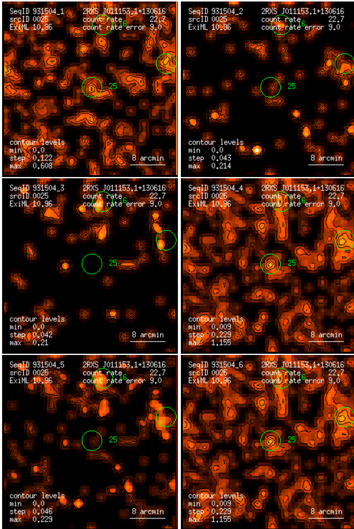
Figure 25: RASS 931504: detection 0025: band rate images, Gaussian filter: (1) PSPC channels 11 – 41, (2) 52 – 90, (3) 91 – 201, (4) 11 – 235, (5) 52 – 201, (6) 11 – 201. Broad band rates in counts/ks. Band rate contour levels in counts/ks/arcmin 2 .
