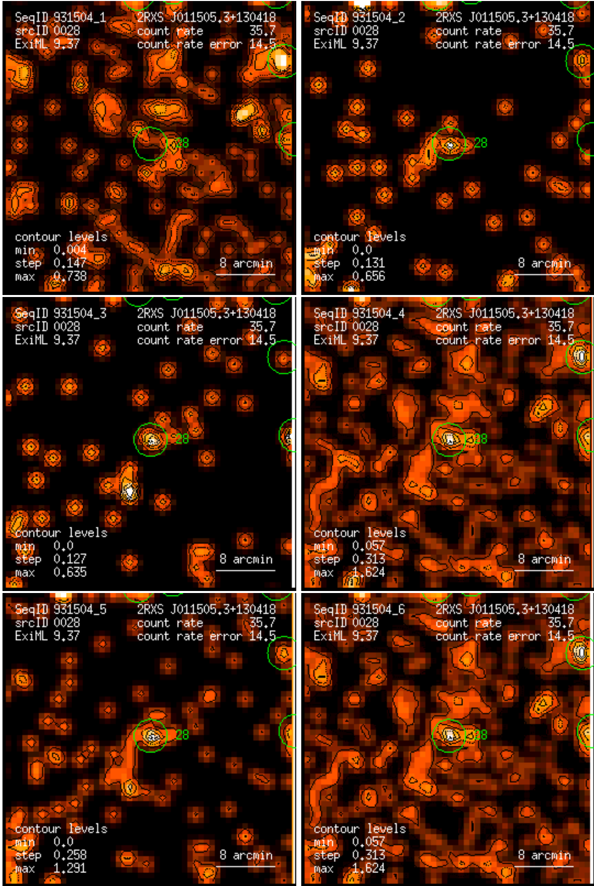
Figure 28: RASS 931504: detection 0028: band rate images, Gaussian filter: (1) PSPC channels 11 – 41, (2) 52 – 90, (3) 91 – 201, (4) 11 – 235, (5) 52 – 201, (6) 11 – 201. Broad band rates in counts/ks. Band rate contour levels in counts/ks/arcmin 2 .
