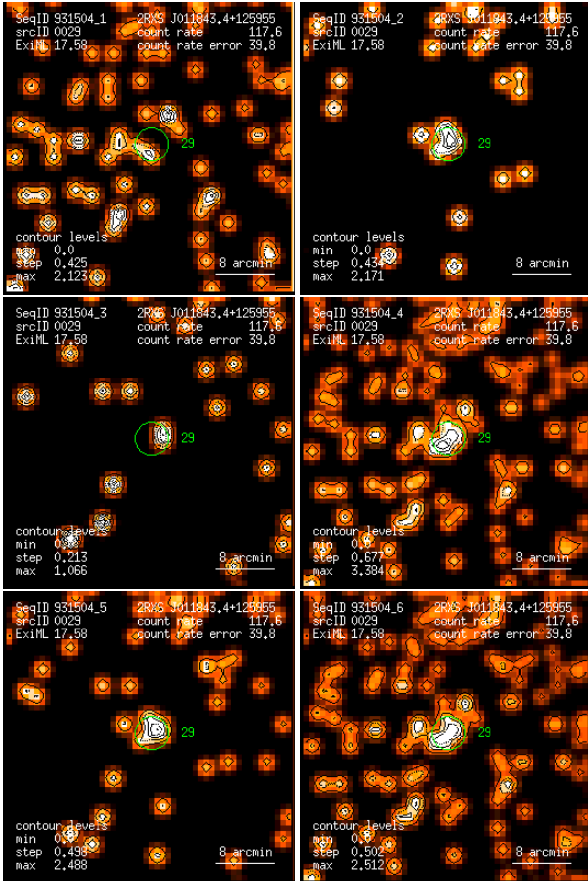
Figure 29: RASS 931504: detection 0029: band rate images, Gaussian filter: (1) PSPC channels 11 – 41, (2) 52 – 90, (3) 91 – 201, (4) 11 – 235, (5) 52 – 201, (6) 11 – 201. Broad band rates in counts/ks. Band rate contour levels in counts/ks/arcmin 2 .
