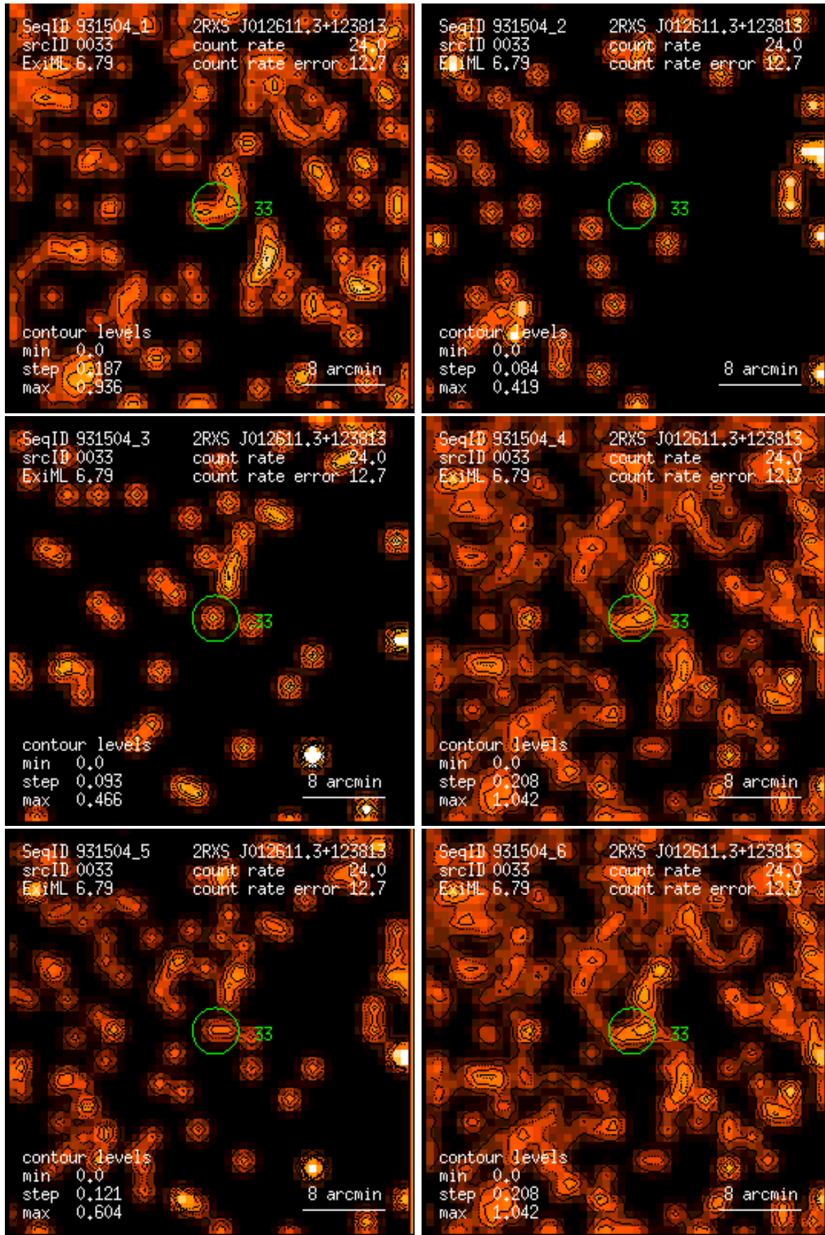
Figure 33: RASS 931504: detection 0033: band rate images, Gaussian filter: (1) PSPC channels 11 – 41, (2) 52 – 90, (3) 91 – 201, (4) 11 – 235, (5) 52 – 201, (6) 11 – 201. Broad band rates in counts/ks. Band rate contour levels in counts/ks/arcmin 2 .
