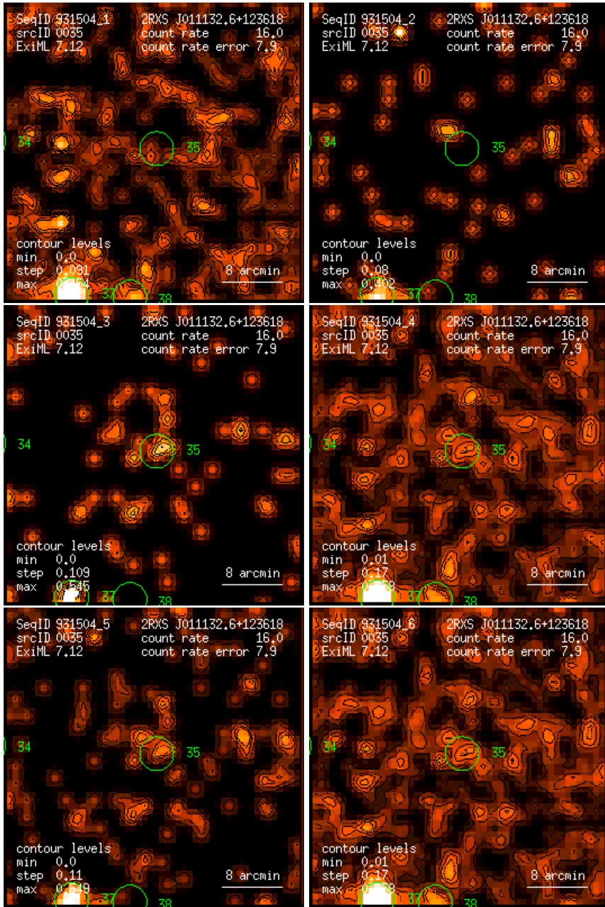
Figure 35: RASS 931504: detection 0035: band rate images, Gaussian filter: (1) PSPC channels 11 – 41, (2) 52 – 90, (3) 91 – 201, (4) 11 – 235, (5) 52 – 201, (6) 11 – 201. Broad band rates in counts/ks. Band rate contour levels in counts/ks/arcmin 2 .
