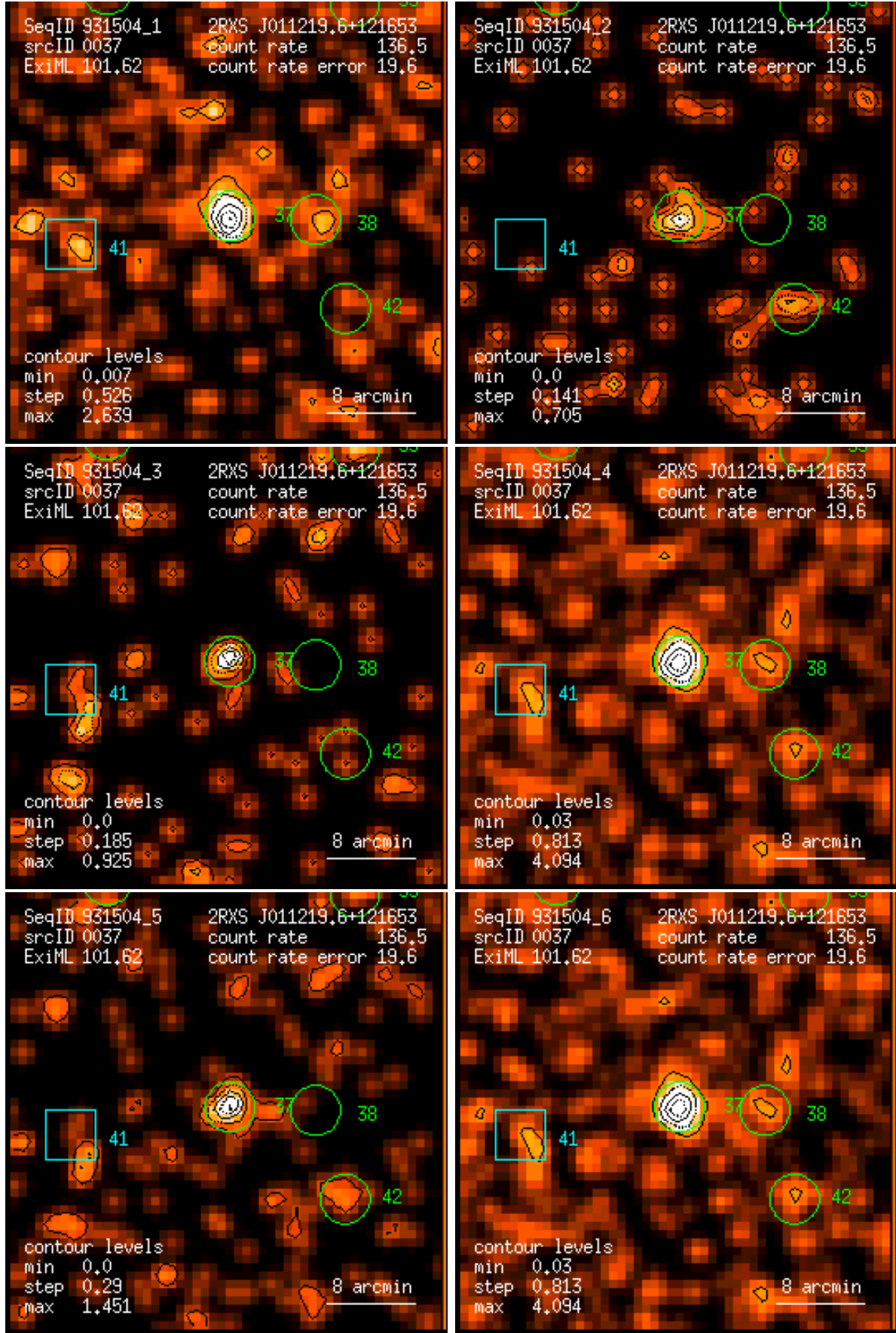
Figure 37: RASS 931504: detection 0037: band rate images, Gaussian filter: (1) PSPC channels 11 – 41, (2) 52 – 90, (3) 91 – 201, (4) 11 – 235, (5) 52 – 201, (6) 11 – 201. Broad band rates in counts/ks. Band rate contour levels in counts/ks/arcmin 2 .
