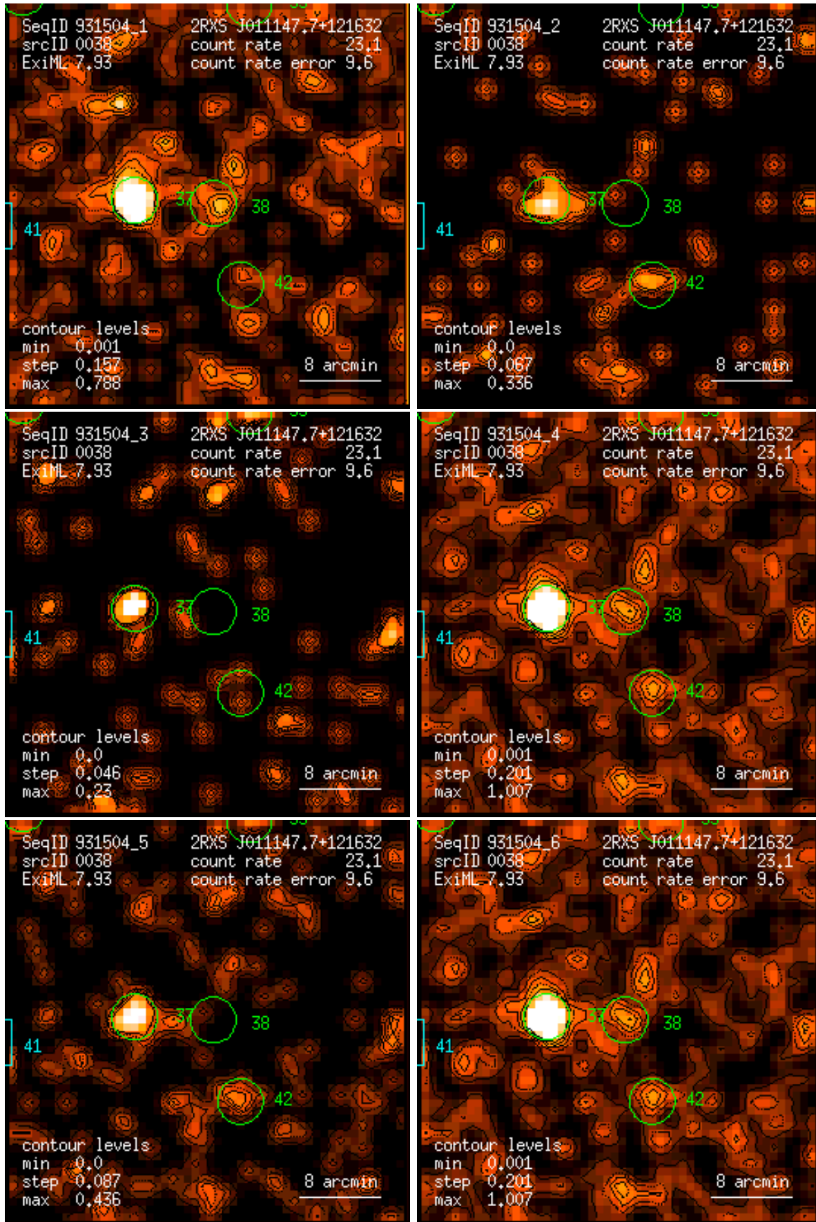
Figure 38: RASS 931504: detection 0038: band rate images, Gaussian filter: (1) PSPC channels 11 – 41, (2) 52 – 90, (3) 91 – 201, (4) 11 – 235, (5) 52 – 201, (6) 11 – 201. Broad band rates in counts/ks. Band rate contour levels in counts/ks/arcmin 2 .
