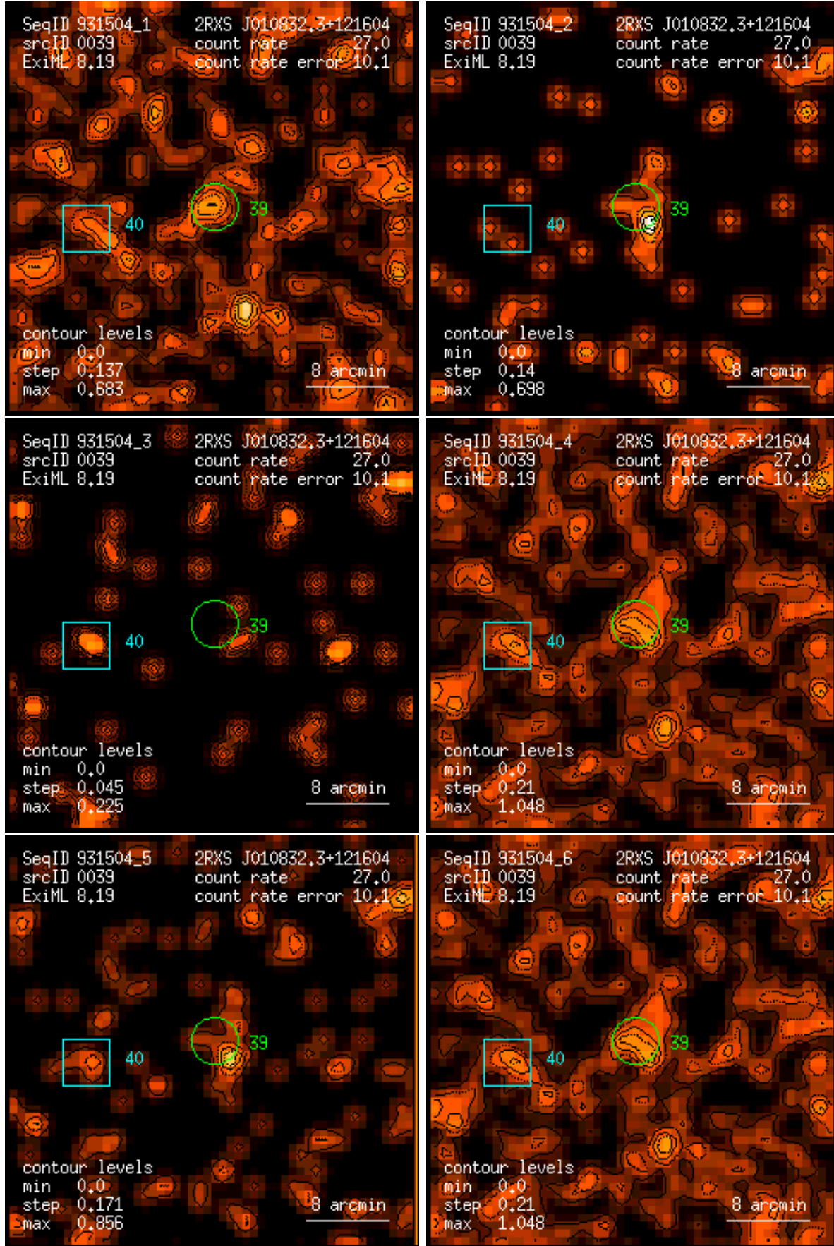
Figure 39: RASS 931504: detection 0039: band rate images, Gaussian filter: (1) PSPC channels 11 – 41, (2) 52 – 90, (3) 91 – 201, (4) 11 – 235, (5) 52 – 201, (6) 11 – 201. Broad band rates in counts/ks. Band rate contour levels in counts/ks/arcmin 2 .
