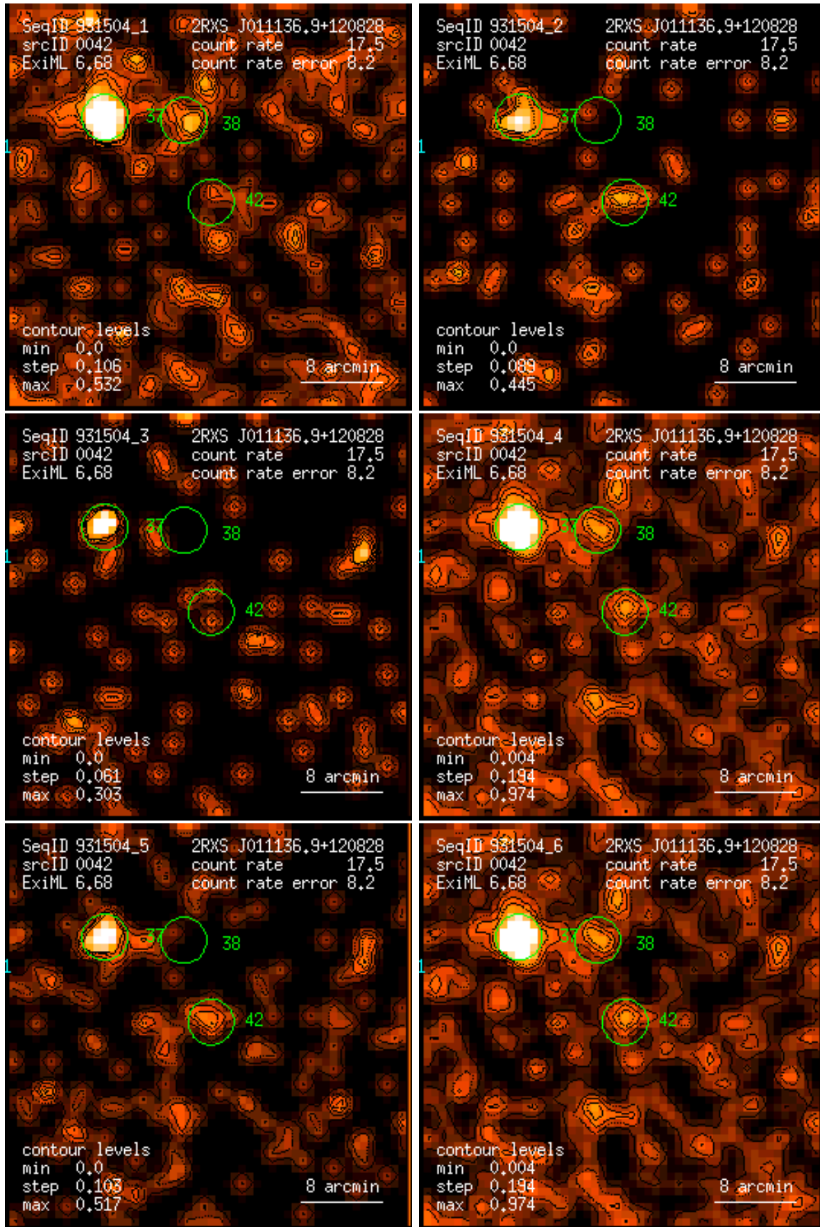
Figure 42: RASS 931504: detection 0042: band rate images, Gaussian filter: (1) PSPC channels 11 – 41, (2) 52 – 90, (3) 91 – 201, (4) 11 – 235, (5) 52 – 201, (6) 11 – 201. Broad band rates in counts/ks. Band rate contour levels in counts/ks/arcmin 2 .
