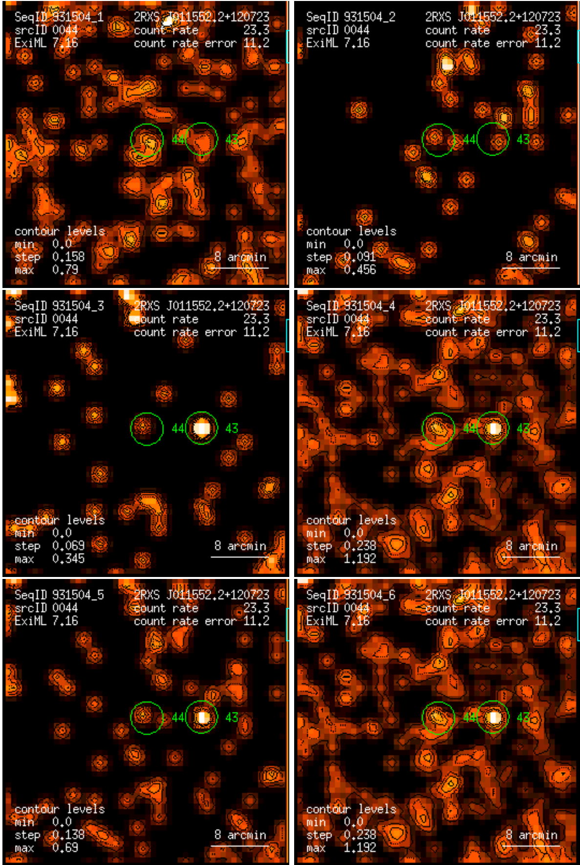
Figure 44: RASS 931504: detection 0044: band rate images, Gaussian filter: (1) PSPC channels 11 – 41, (2) 52 – 90, (3) 91 – 201, (4) 11 – 235, (5) 52 – 201, (6) 11 – 201. Broad band rates in counts/ks. Band rate contour levels in counts/ks/arcmin 2 .
